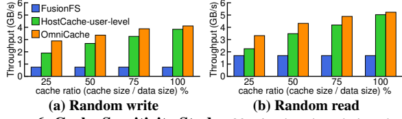
Figure 6: Cache Sensitivity Study. 32 microbenchmark threads with different cache ratio from 25% to 100% (maintaining equal total cache size for HostCache-user-level and OmniCache ).
