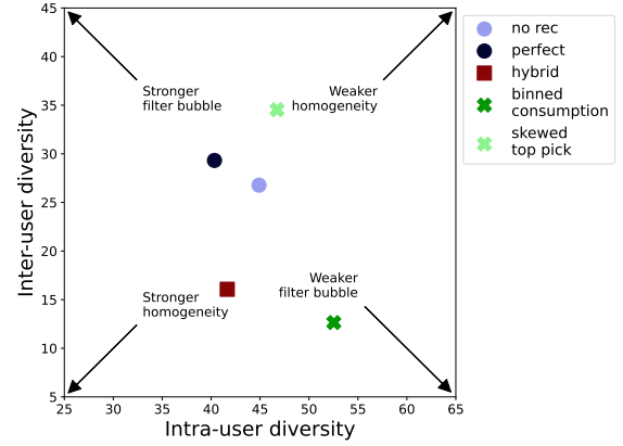
Figure 6: Inter-user diversity vs. intra-user diversity for different recommendation algorithms. As shown here, binned consumption-based recommendation greatly increases intra-user diversity and reduces inter-user diversity compared to no recommendation by exposing users towards the popular items from each genre. Skewed top pick recommendation with \delta = 1 increases inter-user and intra-user diversity simultaneously compared to no recommendation by exposing near-mode users more towards niche items.
