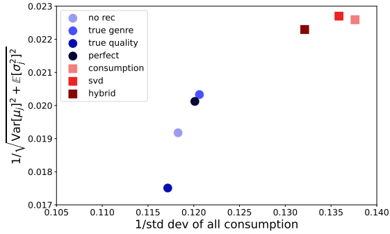
Figure 2: Our definition of homogeneity, formally given by 1/\sqrt{\text{inter-user diversity}^2 + \text{intra-user diversity}^2} , vs. the inverse of the standard deviation of all consumption for each of the seven recommendation algorithms. The Pearson correlation coefficient between the two values is 0.93, i.e. they are highly correlated.
