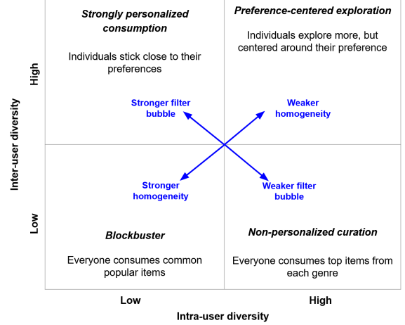
Figure 1: Identifying the strength of homogeneity and filter bubble effect for different levels of inter-user and intra-user diversity. The dynamics seen here motivate our novel definitions of homogeneity and the filter bubble effect.
