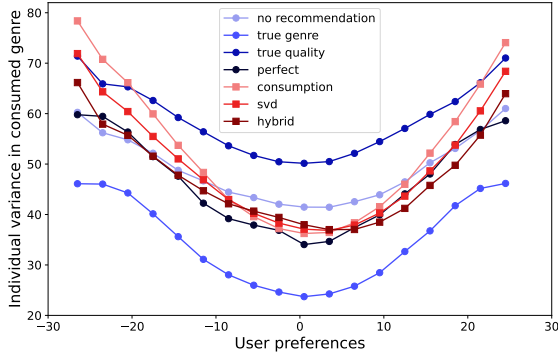
Figure 5: Consumed genre variance (see section 4) against user preferences for the recommendation algorithms in section 5.1. Compared to no recommendation, past consumption-based recommendations decrease variance for near-mode users and increase variance for niche users by pushing everyone towards blockbuster items.
