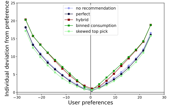
Figure 7: Deviation between mean consumed genre (see section 4) and preference vs. preferences for different recommendations. As shown here, binned consumption-based recommendation causes deviations similar to past consumption-based recommendation. Since every user consumes the popular items from each genre, everyone's mean consumed genre gets close to 0. Skewed top pick recommendation with \delta = 1 causes less deviation compared to no recommendation. It keeps niche users close to their preferences, while exposing near-mode users to niche items from both sides of the mode.
