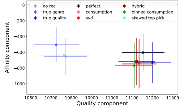
Figure 12: Breakdown of mean individual utility into quality and affinity components for two novel recommendations, as well as for no recommendation, perfect recommendation and hybrid recommendation. As shown here, binned consumption recommendation performs similarly to past consumption-based recommendations. On the other hand, since skewed top pick recommendation prioritizes exploration over anything else, its performance is significantly worse, and comparable to no recommendation.
