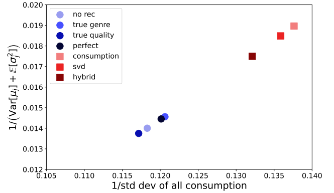
Figure 11: 1/(\text{inter-user diversity} + \text{intra-user diversity}) against the inverse of the standard deviation of all consumption for each of the seven recommendation algorithms. The Pearson correlation coefficient between the two values is 0.99992089, i.e. they are highly correlated.
