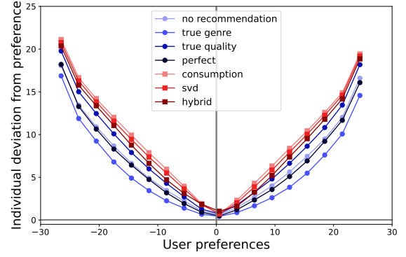
Figure 4: Deviation between mean consumed genre (see section 4) and preference vs. preferences for the recommendation algorithms. Compared to no recommendation, past consumption-based recommendations cause large deviations in mean consumed genre towards 0, by pushing all users towards items with near-mode genres.
