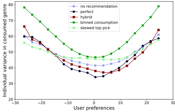
Figure 8: Consumed genre variance (see section 4) against user preferences for two novel recommendations, as well as for no recommendation, perfect recommendation and hybrid recommendation. binned consumption-based recommendation significantly increases variance for everyone by pushing everyone towards the popular items from each genre. Skewed top pick recommendation increases variance for near-mode users by pushing them towards more niche items.
