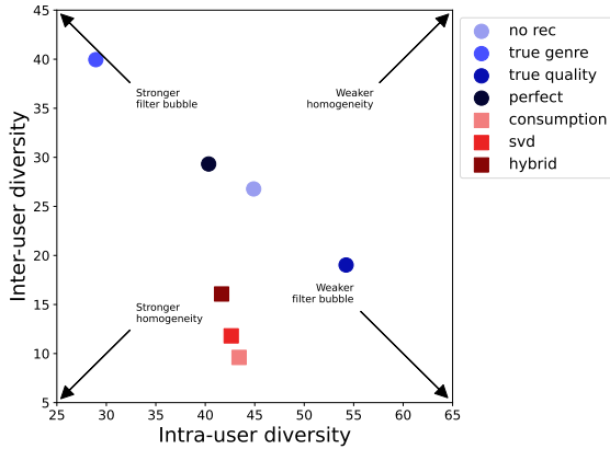
Figure 3: Inter-user diversity vs. intra-user diversity for the different recommendation algorithms. As shown, the baseline algorithms induce a direct trade-off between the two types of diversity. Past consumption-based recommendation algorithms deviate from this trade-off line primarily by reducing inter-user diversity—they do not significantly affect intra-user diversity.
