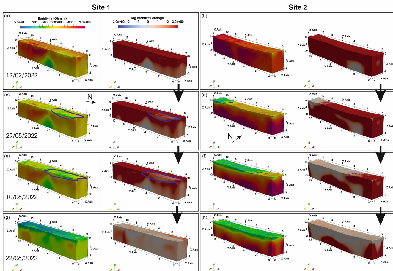
Figure 3. In (a), (c), (e), and (g) is shown a 3D model of absolute electrical resistivity values on the left-hand side and resistivity change relative to ERT data recorded on 2 August 2021 on the right-hand side, corresponding to Site 1. In (b), (d), (f), and (h) is shown a 3D model of absolute electrical resistivity values on the left-hand side and resistivity change relative to ERT data recorded on 2 August 2021 on the right-hand side, corresponding to Site 2. Axes are in metres. The purple line delineates zones of interest where changes in resistivity are detected.
