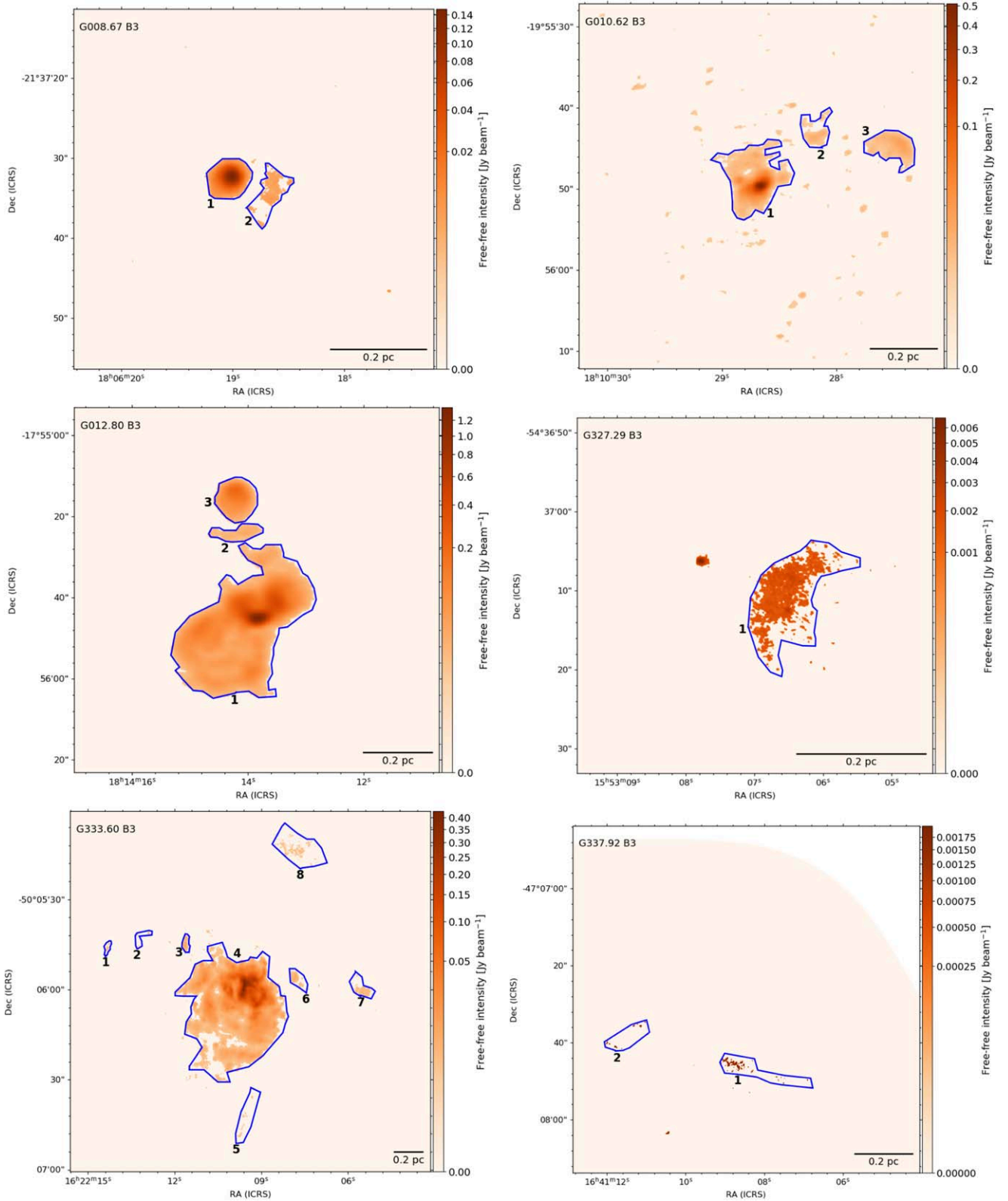
Figure 2. Free-free estimation maps in Band 3 for protoclusters G008.67 (top left), G010.62 (top right), G012.80 (second left), G327.29 (second right), G333.60 (third left), G337.92 (third right), G351.77 (fourth left), G353.41 (fourth right), W43-MM2 (fifth left), W43-MM3 (fifth right), W51-E (bottom left), and W51-IRS2 (bottom right). The compact emission at the center of G327.29 is dominated by contamination from molecular lines (see Section 3.3).
