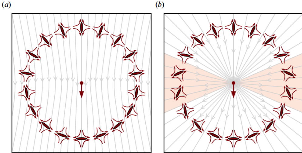
Figure 3. Mechanism of the instability: a point force generates in-plane velocity u (grey streamlines). The magenta streamlines depict the symmetric part of the local, linear flow field around particles at a distance r . Particles are shown in their most favoured orientation, with their long axis parallel to the extensional component of the flow field generated by the point force. (a) For \ell \gg r (membrane-dominated regime), neighbours always reorient such that they are drawn towards the point force, thereby increasing particle density. (b) By contrast, at much longer length scales r \gg \ell (subphase-dominated regime), particles that fall within the shaded region reorient such that they are drawn away from the point force, reducing particle density and stabilizing the suspension. For a fixed \eta_s and \eta , the system transitions continuously from membrane-dominated to subphase-dominated at large enough distances.
