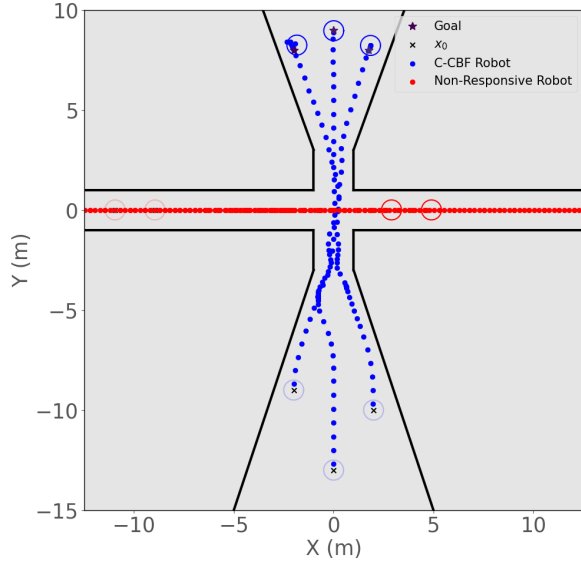
Fig. 2: XY paths for the warehouse robots (blue) and non-responsive agents (red) in the warehouse control problem.
