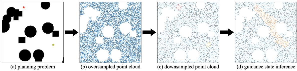
Fig. 2: Guidance state inference by point-based network. Red is start, yellow is goal, blue is free states, and orange is guidance states.
