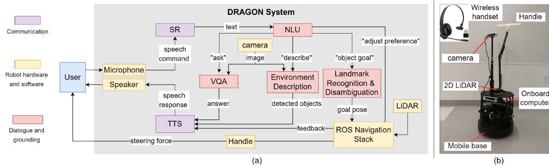
Fig. 2. Overview of the system and platform of DRAGON. (a) Submodules, message passing, and user interface. (b) The robot platform.
