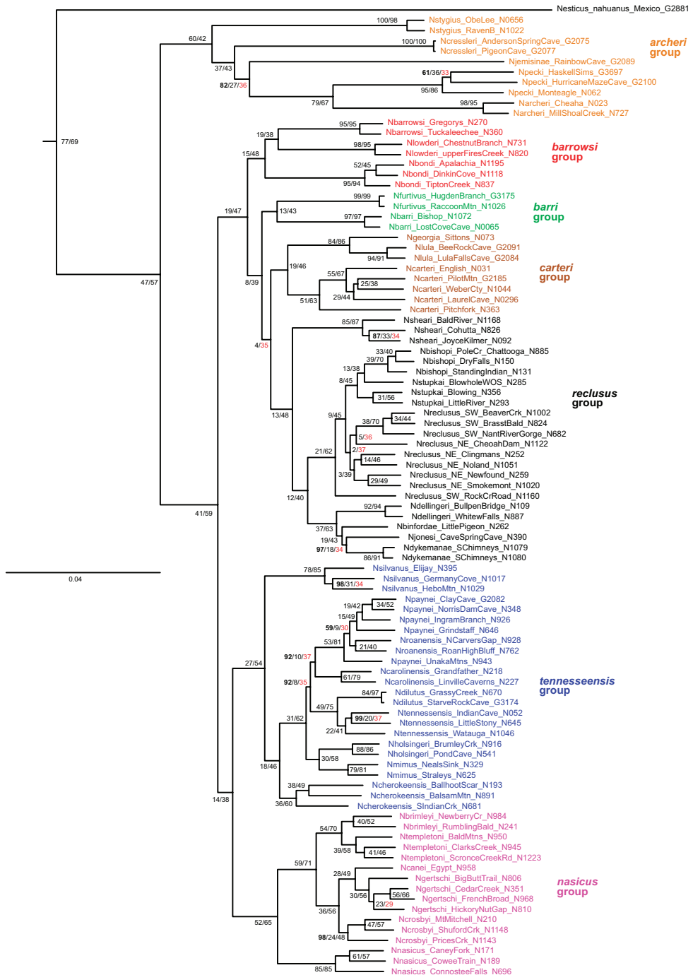
Figure 3. UCE concatenated maximum likelihood tree. Distant outgroups removed (for graphical purposes), specimen numbers correspond to those in Suppl. material 3 (with detailed location provided in Suppl. material 1). Node numbers correspond to bootstrap (bold text) / gCF / sCF. Only bootstrap values below 100 shown, all others 100. gCF and sCF values rounded to nearest integer; sCF values below 38 highlighted with red text.
