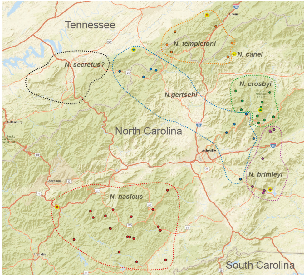
Figure 30. Distribution of nasicus group species. Type localities designated with yellow circles. Primary cities shown for geographic context. Dashed lines circumscribe known species distributions; possible distribution of Nesticus secretus is tentative, see text for details.
