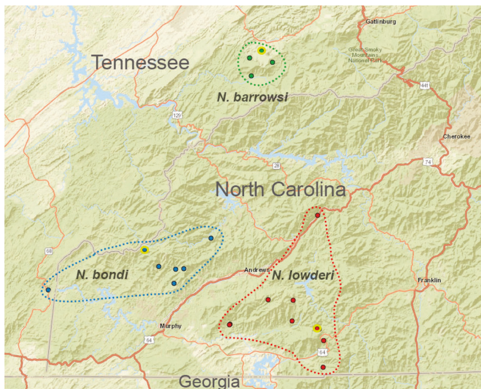
Figure 42. Distribution of the barrowsi group. Type localities designated with yellow circles. State boundaries and major cities shown for geographic context. Dashed lines circumscribe known species distributions.
