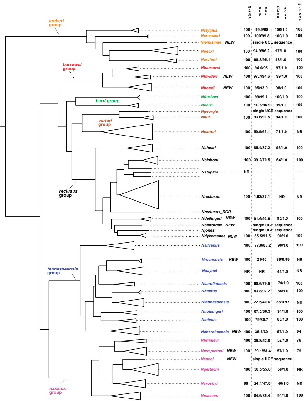
Figure 5. Summary species tree (from UCE topologies), with summary statistics for species support. Branch lengths are arbitrary. New species highlighted. NR = not recovered as clade.
