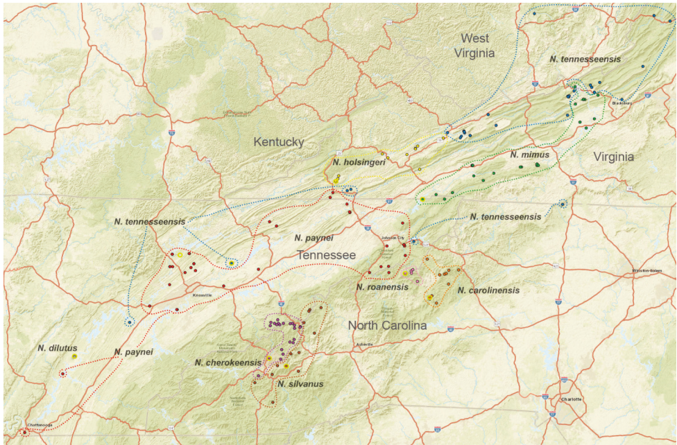
Figure 13. Distribution of tennesseensis group species. Type localities designated with yellow circles. State boundaries and major cities shown for geographic context. Dashed lines circumscribe known species distributions.
