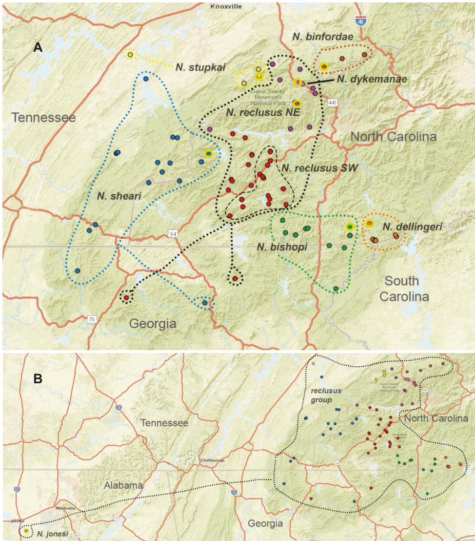
Figure 53. A distribution of reclusus group species B distribution of Nesticus jonesi . Type localities designated with yellow circles. State boundaries and major cities shown for geographic context. Dashed lines circumscribe known species distributions. The geographic distribution of “ N. cooperi -like” populations is circled; this includes some female-only locations which are inside this distribution and included here only for purposes of graphical convenience.
