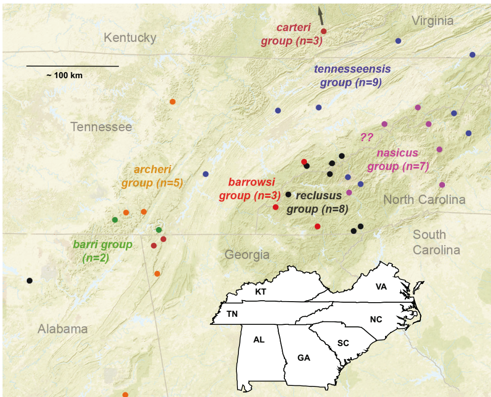
Figure 7. Map of all type localities. Type locality for Nesticus secretus is geographically uncertain (see text), designated with a question mark. Inset map shows full map for US states of interest. Scale bar: approximately 100 kilometers.
