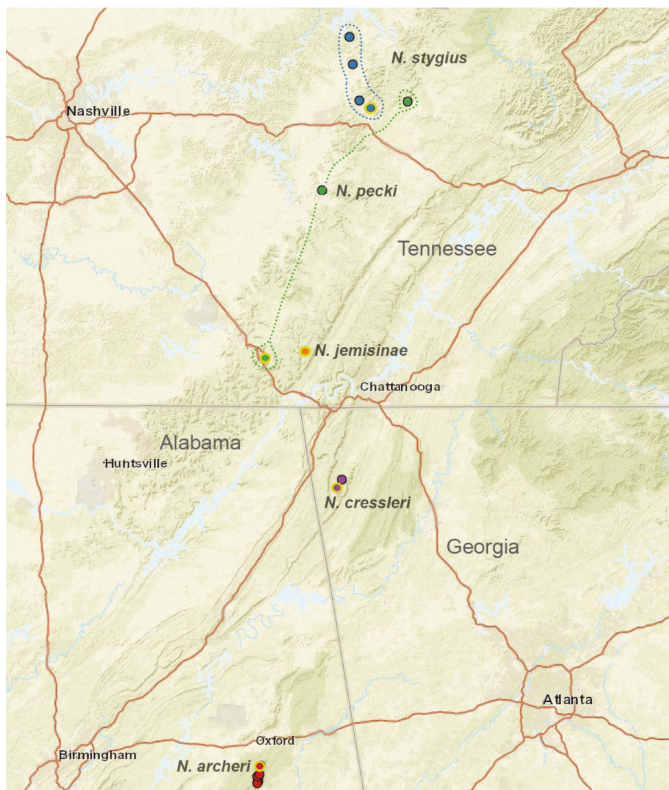
Figure 8. Distribution of the archeri group, including Nesticus archeri , N. pecki , N. jemisiae , N. cressleri , and N. stygius . State boundaries and major cities shown for geographic context. Dashed lines circumscribe the distributions of N. pecki and N. stygius .
