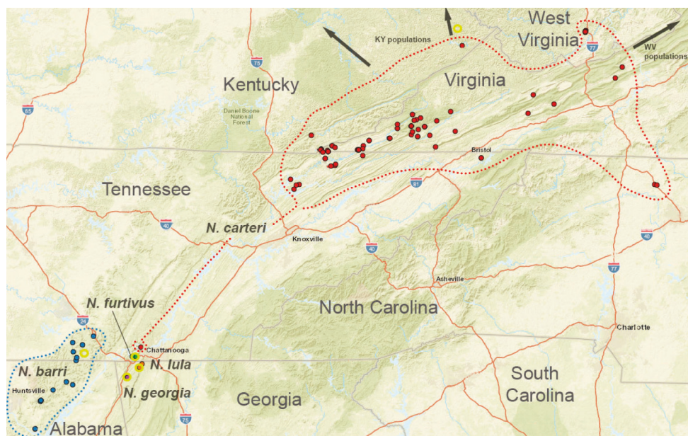
Figure 49. Distribution of barri and carteri groups. Type localities designated with yellow circles. State boundaries and major cities shown for geographic context. Dashed lines circumscribe known species distributions.
