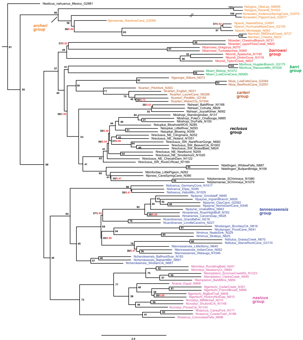
Figure 4. UCE ASTRAL species tree. Distant outgroups removed (for graphical purposes), specimen numbers correspond to those in Suppl. material 3 (with detailed location provided in Suppl. material 1). Included are quartet support values (rounded to nearest integer), and local posterior probability values (if less than 1.0, red text). Branch lengths in coalescent units for internal branches only, terminal branch lengths arbitrary. Internal branch to Nesticus cressleri truncated for graphical purposes.
