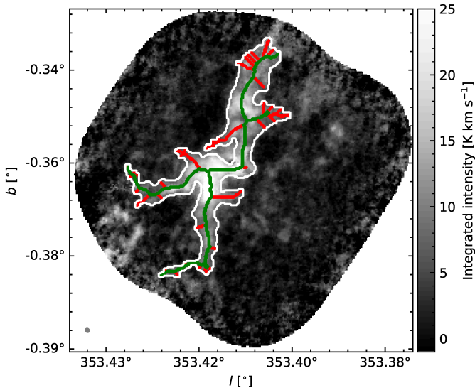
Fig. A.1: FilFinder filamentary identification. The background indicates the moment 0 map of the extracted \text{N}_2\text{H}^+ isolated components. The white contour shows the area where FilFinder identifies multiple filamentary structures (red and green lines). We remove the small-scale structures (in red) by “pruning” the skeleton structure from medskel, obtaining the main filaments of G353. We represent these filaments with green lines.
