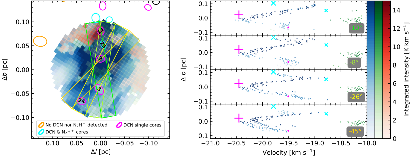
Fig. 11. Left panel: integrated intensity map of the modeled \text{N}_2\text{H}^+ isolated component within a region of radius of 0.1 pc, centered at V-shape “C”. With boxes in shades of green and yellow, we indicate the different paths taken to create the PV diagrams shown on the right panel. The area covered by these four PVs matches the extent of this V-shape (see Fig. 12). The 1.3 mm cores are indicated using the same convention from Fig. 9. For the cores within the radius of 0.1 pc we indicate their IDs in black. Right panel: PV diagrams associated with the colored rectangles in the left panel. At the bottom right corner of each sub panel, with colored values, we indicate the angle (counter-clockwise) of each PV path. The PV paths match the V-shape coverage (right panel of Fig. 12). We see the overall structure of this V-shape persists at different angles, indicating that these structures are not a result of projection in the POS.
