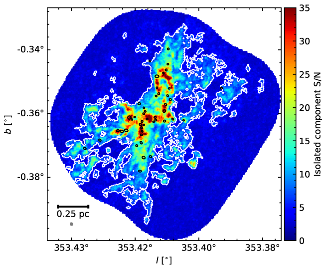
Fig. 3. G353 N_2H^+ isolated component S/N map. The white contour indicates the location of data with an isolated component S/N \geq 5 . We show the location of the 1.3 mm cores presented in Louvet et al. (2024) with black ellipses and are located in regions with S/N \geq 15 . We indicate the beam size of these data with a gray ellipse at the bottom left corner. Outside the S/N contour we make a rough extraction of the isolated component (see text). For data inside the S/N contours, we implement a procedure based on detection of peaks and valleys, to individually extract high ( \geq 5 ) S/N isolated components (see Sect. 3).
