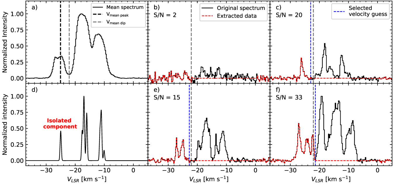
Fig. 2. N_2H^+ spectra involved in our isolated component extraction procedure. Panel a: normalized average N_2H^+ spectrum (solid black line) over the entire region. We show the location of the mean peak of the isolated component (dashed black line) and the “mean dip” (dashed gray line), see text. Middle and right panels: normalized example spectra (within a pixel) of the N_2H^+ isolated velocity component extraction procedure (see Sect. 3). We show G353 N_2H^+ spectra with solid black lines and the extracted isolated component, along with emission-free channels, with dashed red lines. Panel d: expected N_2H^+ emission for an excitation temperature of 15 K, an opacity of 1, velocity centroid of -17 km s ^{-1} , and a line width of 0.2 km s ^{-1} . We see the seven hyperfine components characteristic of this tracer, in which the most blueshifted corresponds to the isolated component. To derive this emission we use “n2hp_vtau” model from PySpecKit. In panels b, c, e, and f) we indicate V_{mean\ dip} with a dashed gray line. We present data with S/N < 5 in panel b, in which we make a rough extraction based on the V_{mean\ dip} . We show data with S/N \geq 5 in panels c, e, and f, presenting clear single, double, and triple N_2H^+ isolated velocity components, respectively. In these examples we represent the selected velocity guess that separates the isolated component emission from the main line emission with dashed blue lines. The offset positions ( \Delta l , \Delta b ) of the spectra in panels b, c, e, and f are (0.68 pc, 0.27 pc), (0.12 pc, -0.28 pc), (-0.08 pc, 0.47 pc), and (0.16 pc, -0.07 pc), respectively. These offsets are estimated relative to the center of the region (see Sect. 1).
