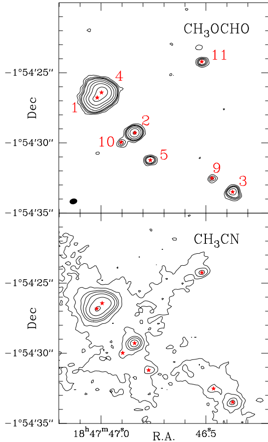
Fig. 5. Top: methyl formate intensity map integrated over the velocity (bandwidth of 25 \text{ km s}^{-1} around the 216.21 \text{ GHz} transitions). The contours correspond to 3, 6, 9, 12, 24, 50, 100, and 200 \sigma , where the rms noise \sigma = 2.6 \text{ K km s}^{-1} . Bottom: Methyl cyanide intensity map integrated over the velocity (bandwidth of 120 \text{ km s}^{-1} around the 91.97 \text{ GHz} transitions). The contours correspond to 5, 10, 20, 30, 50, 100, and 200 \sigma , where the rms noise \sigma = 83 \text{ K km s}^{-1} . The red stars indicate the position of the hot cores identified on Fig. 2.
