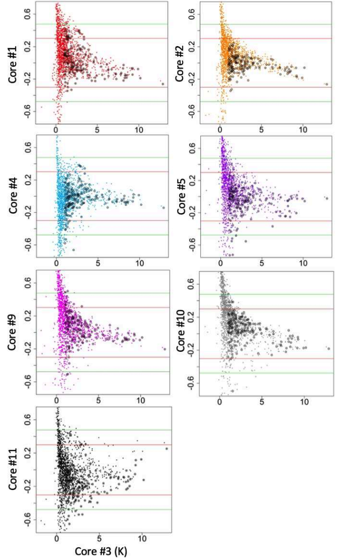
Fig. 15. Logarithm of the normalised ratio R_i = T_i^S / (a_1 \times T_i^{S3}) for cores #1, #2, #4, #5, #9, #10, and #11 versus T_i^{S3} , the channel intensity of the reference source core #3 (see Sect. 6.3). Horizontal red and green lines indicate a departure from R_i = 1 by a factor 2 and 3, respectively. Circles indicate peaks in the core #3 spectrum. Most points right of T_i^{S3} = 2 K remain within a factor of 2 of the linear fit shown in Fig. 13 (slope a_1 ), which indicates a good general similarity in the spectra.
