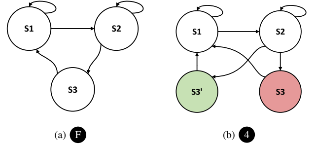
Fig. 3. (a) Example FSM with least-likely state S3 (b) Example FSM with duplicated least-likely state
