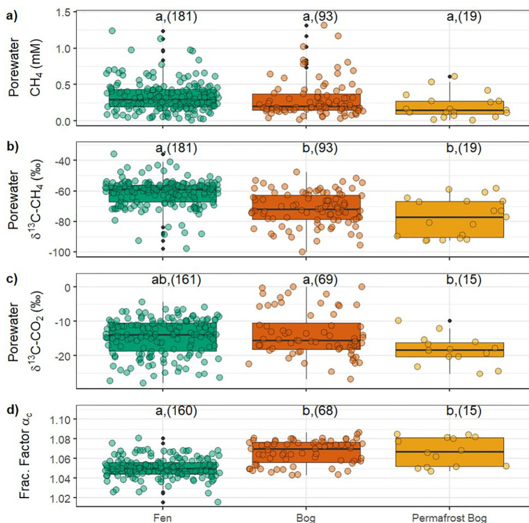
Figure 2. Porewater chemistry across peatland types from all five locations including (a) dissolved \text{CH}_4 , (b) \delta^{13}\text{C}\text{-CH}_4 , (c) \delta^{13}\text{C}\text{-CO}_2 , and (d) the fractionation factor ( \alpha_c ), defined as (\delta^{13}\text{C}\text{-CO}_2 + 1,000)/(\delta^{13}\text{C}\text{-CH}_4 + 1,000) . Colored points represent individual measurements across multiple plots at depths between 0 and 60 cm. Statistical differences (denoted by the letters) were determined using mixed linear regression with individual plots and circumpolar location as random factors to account for multiple samples at each depth and plot and natural variation within the location (significance level 5%; Tukey's HSD: P < 0.05 ). When letters differ between boxes in each row this indicates significant differences. Boxes show 25th to 75th percentiles. Whiskers indicate 10th and 90th percentiles and black points outliers. Horizontal lines denote medians. Sample sizes are indicated next to the letters.
