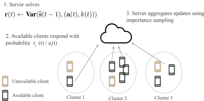
Fig. 1: Illustration of one round of communication of Algorithm 1. (1) Server solves the optimization problem in line 4 and sends the solution to available clients. (2) Available clients in cluster k send an update with probability \frac{r_k(t)}{a_k(t)} (lines 5-12). (3) Server updates the global model with received updates using importance sampling (lines 14-15).
