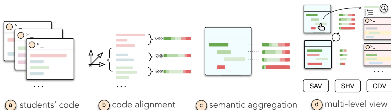
Figure 1: A system overview of CFlow. (a) Upon collecting student code submissions, (b) CFlow extracts and semantically labels the code statements. (c left) These labels are then clustered and represented in a Semantic Aggregation View (SAV). (c right) Statement correctness is color coded and visualized using a stacked bar histogram, forming the Semantic Histogram View (SHV). (d) Users can filter the views by clicking on labels in the SAV or bars in the SHV. The Code Detailed View (CDV) enables for an in-depth inspection of specific code branches.
