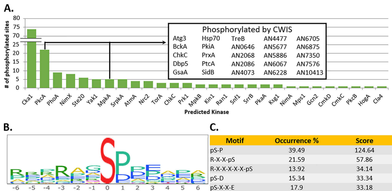
FIG. 5. Overall analysis of dynamic phosphorylation sites. NetworkKIN analysis shows that a majority of the phosphorylation sites are predicted to be phosphorylated by Cka1. PkcA and MpkA (CWIS signaling kinases) phosphorylate multiple proteins showing possible new direct connections to the cell wall repair pathway (A). Motif-logo showing the overall enrichment of amino acids surrounding the phospho-residue, serine, as generated by PHOSIDA (B). Top 5 enriched motifs identified from statistically dynamic phosphosites. The occurrence percent is the relative abundance of the motif in this data set with respect to the proteome and the score is a statistic equivalent to p = 10^{(-\text{score})} (C).
