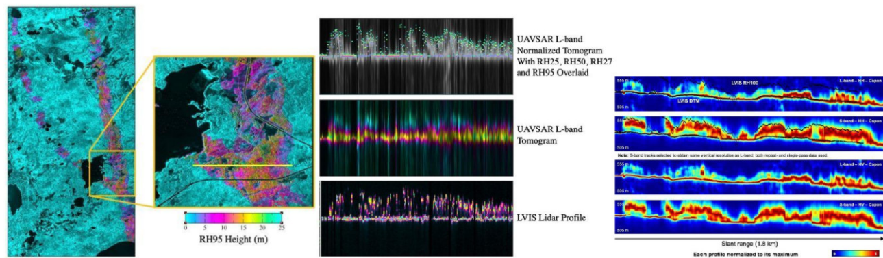
Figure 6. On the left, the location of the transect is shown as a yellow line overlaid on UAVSAR imagery in grayscale and LVIS RH95 data in color where UAVSAR L-band, DLR F-SAR L and S-band and LVIS lidar profiles are compared. The center figure shows UAVSAR L-band tomographic profiles along the transect along with the corresponding LVIS lidar profiles. On the right are the corresponding F-SAR L and S-band tomographic profiles. The L-band radar profiles exhibit power concentrated at the base of the canopy, whereas the LVIS lidar data show more return from the middle portion of the canopy. The S-band obtains greater returns in the upper canopy compared to the L-band and shows more uniform scattering within the canopy.
