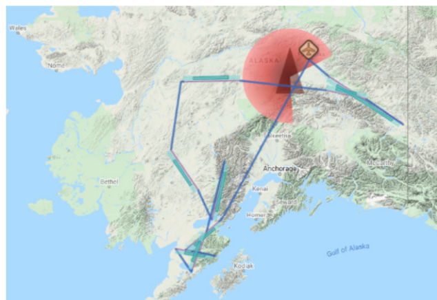
Figure 4. The military radar at Clear, AK, creates a large P-band operations keep-out zone in the central Interior (red areas). The aircraft symbol marks our Fairbanks International Airport (PAFA) base of operations. Data acquisitions (blue bars) are from flight plan 17054. © Google Maps.
