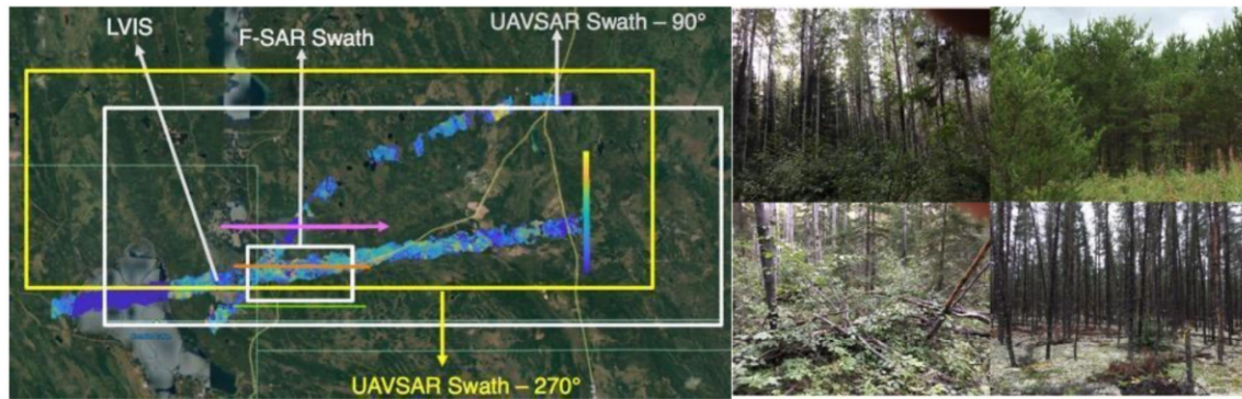
Figure 5. Left: experimental design for the BERMS area TomoSAR flights in August 2018. The large white and yellow boxes show the \sim 18 km wide UAVSAR L-band swaths. The offset is due to the off-nadir viewing angle of the L-band SAR – it is pointed to the south when flying the 270^\circ swath and pointed north when flying the 90^\circ swath. The small white box near the center of the image marks the \sim 3 km wide F-SAR swath. LVIS lidar data are the \sim 1.5 km wide colored swaths across the image; the color scaling reflects the canopy height. Right: photos from 4 of the 17 plots used for in situ ground truth measurement at BERMS. Vegetation at BERMS was mostly jack pine and aspen, with many areas having dense understory vegetation. Most areas have substantial detritus and ground litter left over from previous logging operations. © Google Earth.
