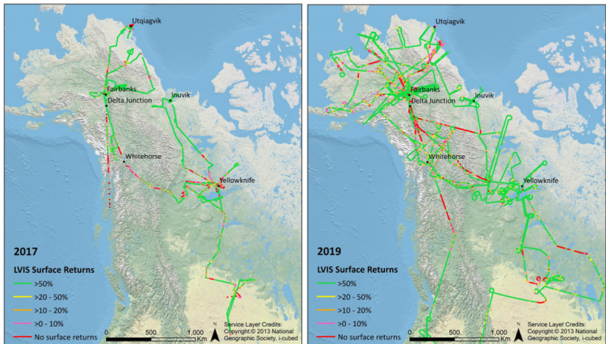
Figure 10. Flight lines for the LVIS 2017 flights (left) and 2019 flights (right) were designed to overlap with the near-field portions of the L-band and P-band SAR swaths to maximize opportunities for synergistic science. Aircraft and weather limited coverage during the 2017 campaign, but complete coverage of the SAR flight lines, was achieved in 2019. These data will enable studies of SAR–lidar fusion over the Arctic–boreal regions as a precursor to NISAR/IceSat-2 studies. © National Geographic Society.
