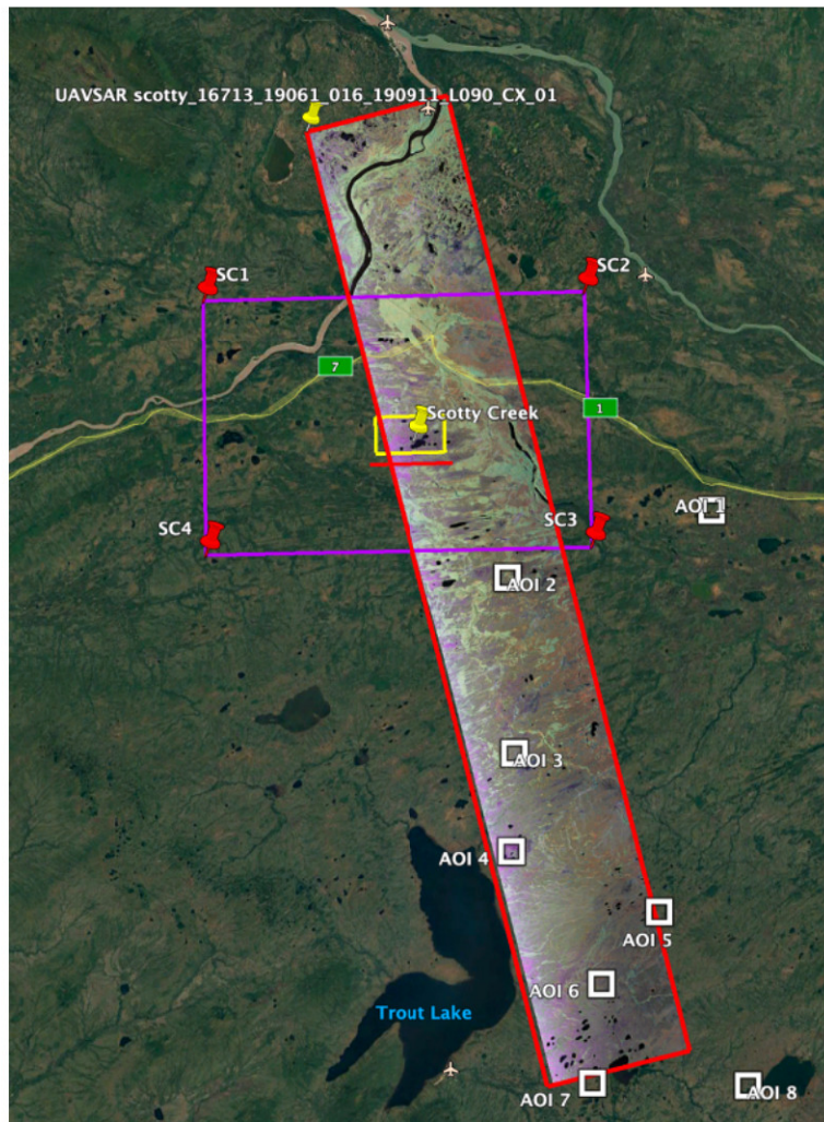
Figure 8. Overlap of the F-SAR acquisition at Scotty Creek, NT (yellow box), and the ABoVE L-band SAR line 16713 (red box and polarized SAR false color). The ABoVE line also captures Scotty Creek AOI 2–6 (see Region C3 details, Sect. 5.3). The SAR data will complement and benefit from the extensive ground-based data acquired in this area (Quinton et al., 2019). © Google Earth.
