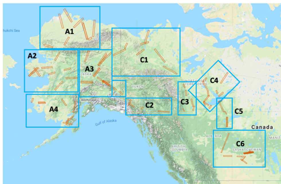
Figure 1. Flight lines for the L-band and P-band PolInSAR measurements capture critical bioclimatic, permafrost, and geographic gradients as well as key field sites and long-term measurement records across the 4 \times 10^6 km 2 ABoVE domain. The flight lines are collected into 10 composites which roughly correspond to the Alaskan (A1–A4) and Canadian (C1–C6) regions sampled on individual flight days. © Google Maps.
