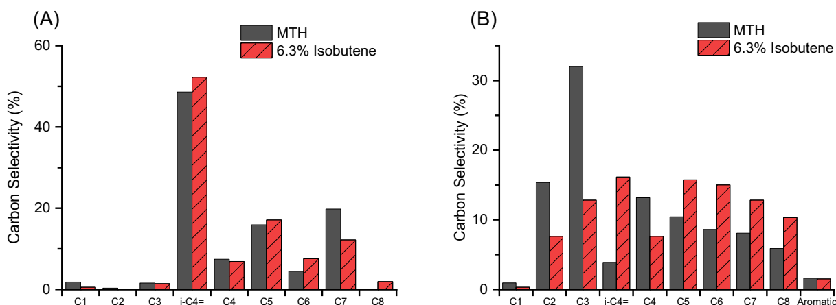
Figure S9 (A) Total carbon selectivity including isobutene over Fe beta for MTH and isobutene co-fed at 300 °C, 0.239 MPa, and WHSV 6.12 g DMEG Catalyst -1 hour -1 , 6.3 % Isobutene co-fed at 216 minutes time on stream. (B) Total carbon selectivity including isobutene over Fe ZSM-5 for MTH and isobutene co-fed at 300 °C, 0.239 MPa, and WHSV 6.12 g DMEG Catalyst -1 hour -1 , 6.3 % Isobutene co-fed at 216 minutes time on stream.
