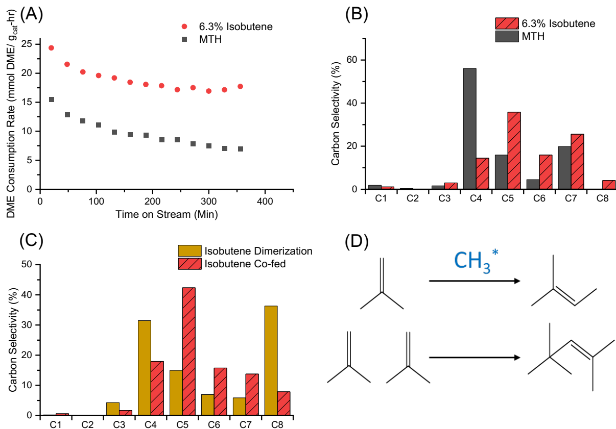
Figure 4 (A) DME consumption rate over H-[Fe]beta for MTH and DME co-fed with isobutene at 300 °C, 0.239 MPa, and WHSV 6.12 g DME /g Catalyst - 1 hour -1 6.3% isobutene co-fed. (B) Carbon selectivity for MTH and DME co-fed with isobutene over H-[Fe]beta after 216 minutes time on stream. (C) Carbon selectivity for isobutene dimerization and isobutene co-fed (24.4%) with DME over H-[Fe]beta after 216 minutes time on stream. Total flow rate and isobutene flow rate are the same for both the co-fed and dimerization reactions. Isobutene, the co-fed olefin, is not accounted for in carbon selectivity due to not being able to differentiate between generated and co-fed isobutene. (D) Isobutene methylation reaction and dimerization reaction. CH 3 * is a surface methoxy group. Carbon balance at 216 minutes time on stream MTH 94%, 6.3% isobutene 95%, and isobutene dimerization 93%.
