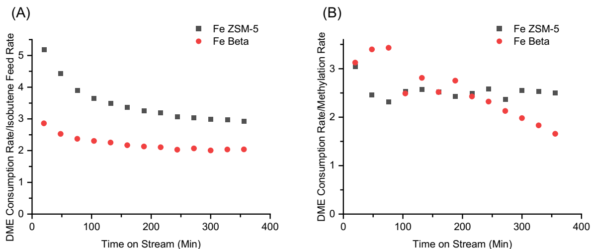
Figure S8 (A) DME consumption rate divided by isobutene feed rate for Fe ZSM-5 and Fe beta with an isobutene co-fed at 300 °C, 0.239 MPa, and WHSV 6.12 g DME /g Catalyst ·h -1 , 6.3 % Isobutene co-fed. (B) DME consumption rate divided by methylation rate for Fe ZSM-5 and Fe beta with an isobutene co-fed at 300 °C, 0.239 MPa, and WHSV 6.12 g DME /g Catalyst ·h -1 , 6.3 % Isobutene co-fed.
