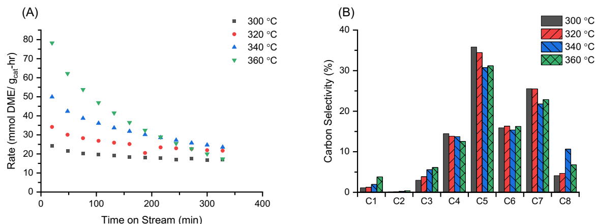
Figure 6 (A) DME consumption rate over H-[Fe]beta for the isobutene co-fed reaction with a 6.3% isobutene co-fed, 0.239 MPa, and WHSV 6.12 g DME /g Catalyst ·h -1 at different temperatures. (B) Carbon selectivity of isobutene co-fed over H-[Fe]beta at different temperatures at 216 minutes time on stream. Carbon balance at 216 minutes time on stream 300 °C 95%, 320 °C 95%, 340 °C 97%, and 360 °C 83%.
