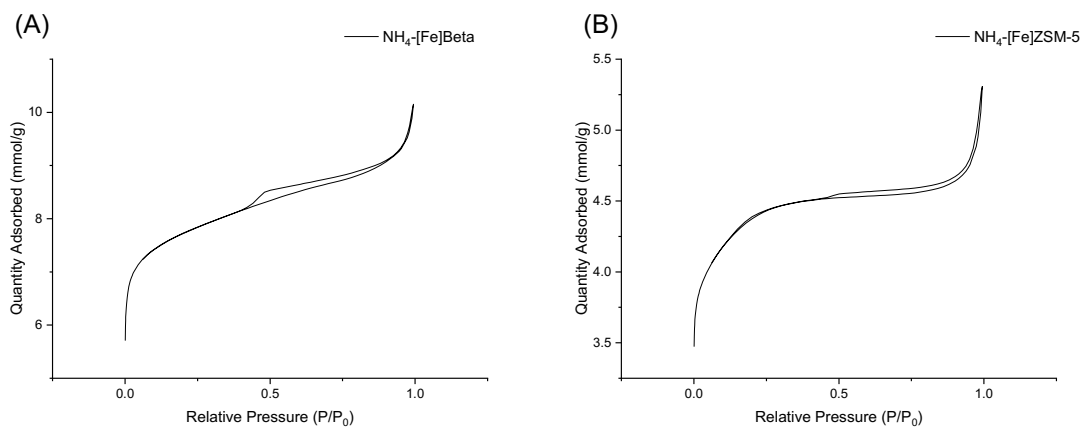
Figure S2 Nitrogen adsorption and desorption Isotherms (A) \text{NH}_4\text{-[Fe]beta} (B) \text{NH}_4\text{-[Fe]ZSM-5}
