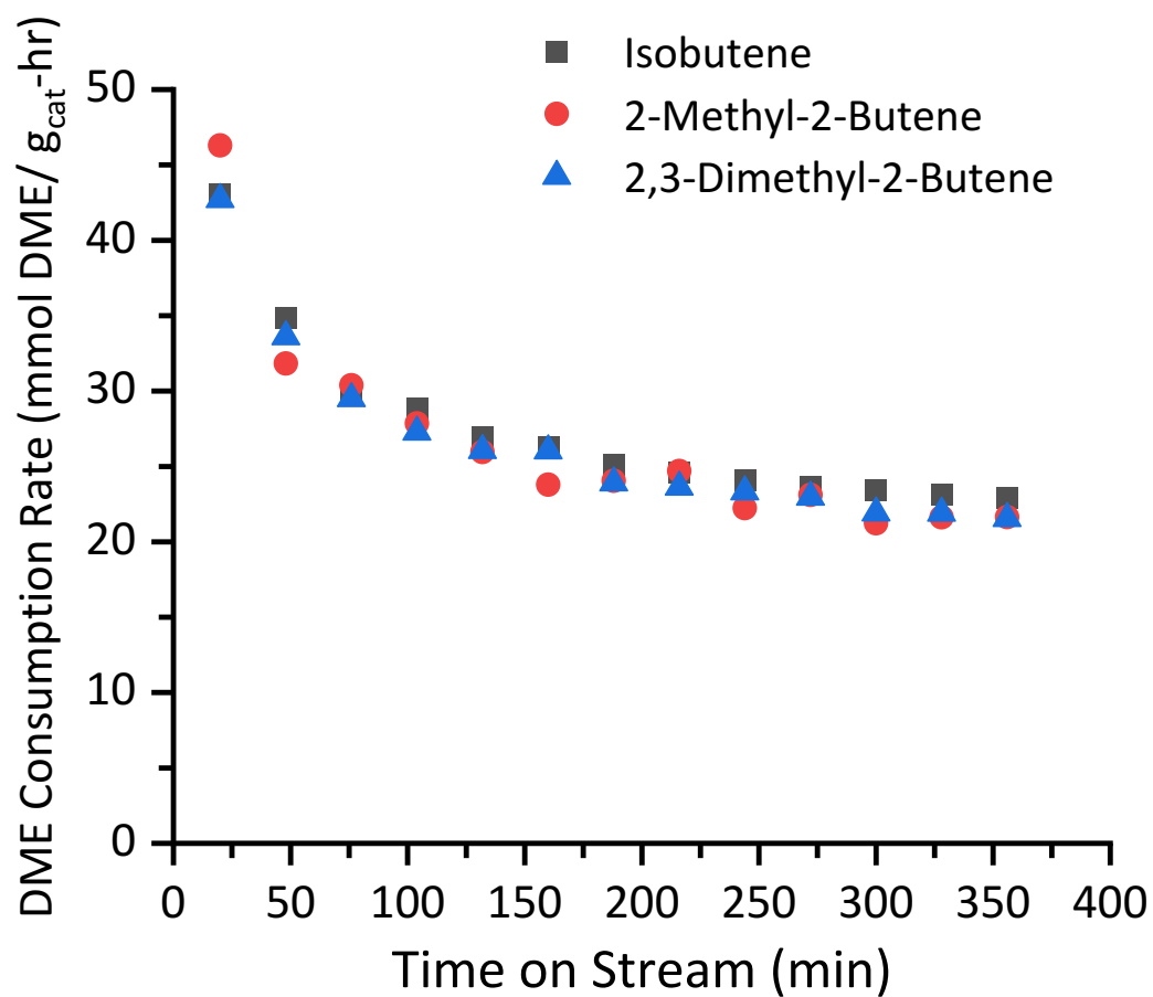
Figure S7 DME consumption rate for different olefin co-feeds over H-[Fe]ZSM-5 at 3.9% olefin co-fed, 300 °C, WHSV 6.12 g DME /g Catalyst hour -1 , and 2.39 bar. Carbon selectivity at 216 minutes time on stream isobutene 93%, 2-methyl-2-butene 94%, and 2,3-dimethyl-2-butene 93%.
