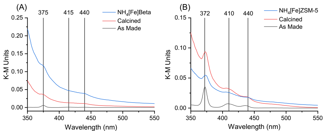
Figure S3 (A) UV/Vis spectra of Fe beta in its as made, calcined, and \text{NH}_4 exchanged form. (B) UV/Vis spectra of Fe ZSM-5 in its as made, calcined, and \text{NH}_4 exchanged form. The vertical black lines correspond to d-d electron transition peaks corresponding to iron (III) in a tetrahedral environment
