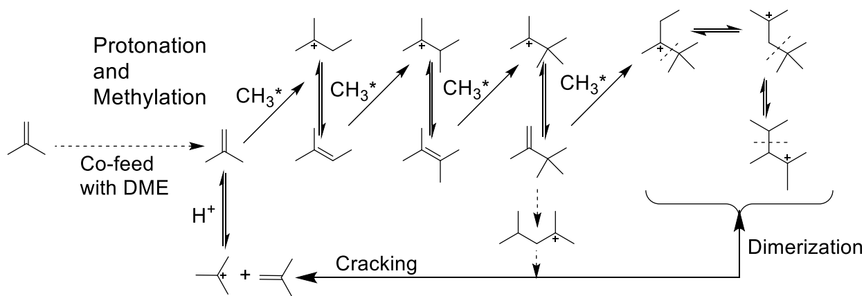
Figure 9 Proposed mechanism of olefin methylation reactions over H-[Fe]beta. \text{CH}_3^* are surface methoxy groups.
