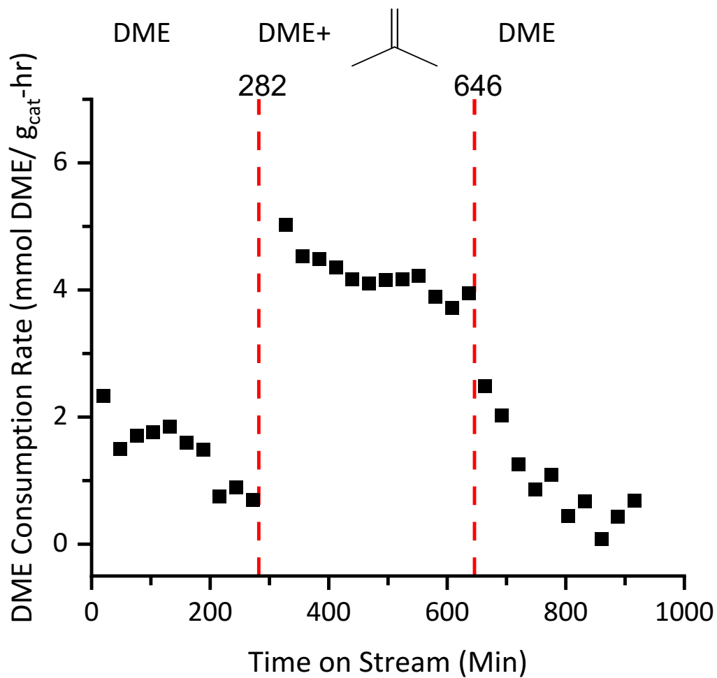
Figure S4 DME consumption rate over H-[Fe]beta at 260 °C showing the effect of the presence or absence of isobutene in the feed. Isobutene is only co-fed between the dashed red lines. H-[Fe]beta at 260 °C, 6.3% isobutene co-fed, WHSV 6.12 g DME /g Catalyst -1 hour -1 and 2.39 bar
