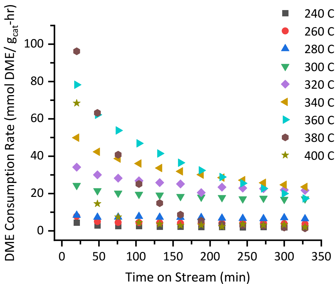
Figure S6 DME consumption rates for 3.9% isobutene co-fed at different temperatures over H-[Fe]ZSM-5 WHSV 6.12 g DME /g Catalyst ·h -1 , and 2.39 bar. Carbon balance after 216 minutes time on stream 240 °C 99%, 260 °C 97%, 280 °C 97%, 300 °C 95%, 320 °C 95%, 340 °C 97%, 360 °C 83%, 380 °C 91%, 400 °C 100%. At 400 °C the carbon balance was 76% at 20 min time on stream and 91% at 48 min time on stream.
