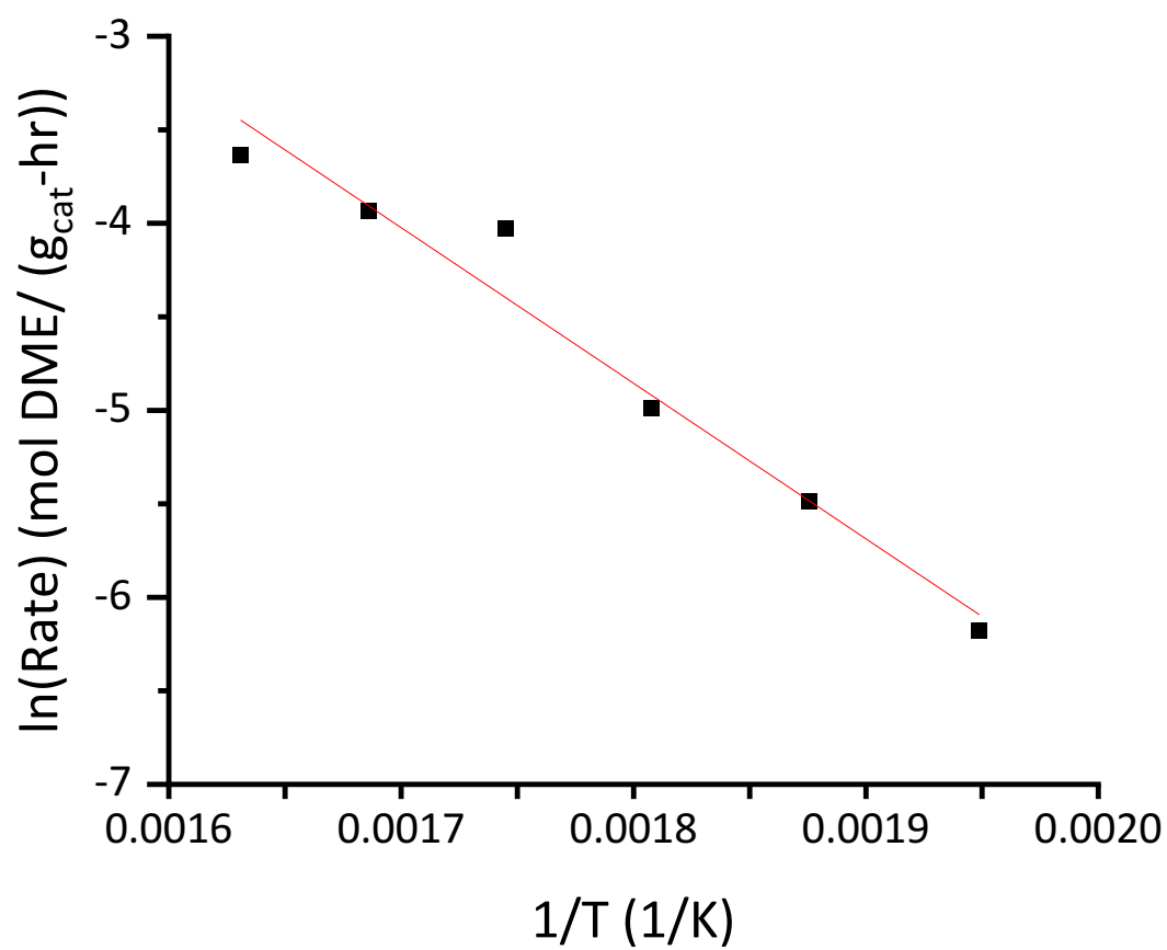
Figure S5 Arrhenius plot for isobutene co-fed reaction
