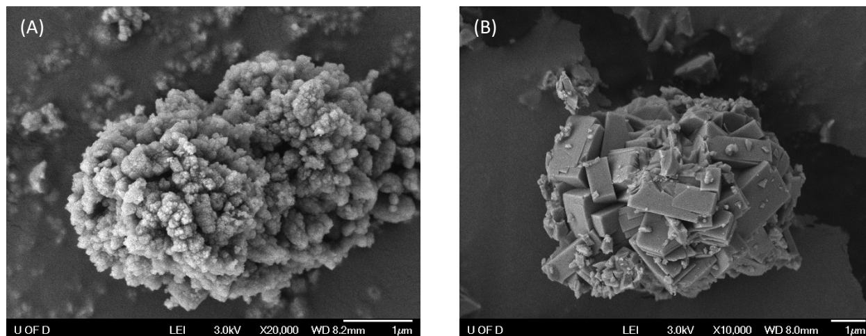
Figure 3 SEM Images of Iron Zeolites (A) \text{NH}_4[\text{Fe}]\beta (B) \text{NH}_4[\text{Fe}]\text{ZSM-5}
