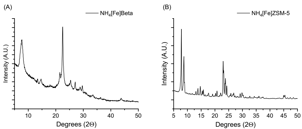
Figure S1 (A) XRD pattern of \text{NH}_4[\text{Fe}]\text{Beta} (B) XRD pattern of \text{NH}_4[\text{Fe}]\text{ZSM-5}
