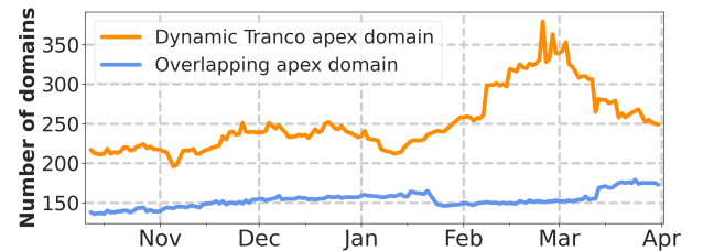
Figure 10: Number of domains that both activate HTTPS records and use non-Cloudflare name servers.
