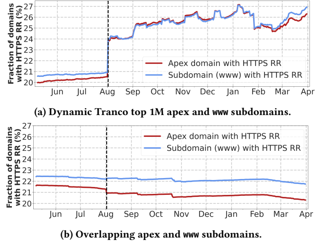
Figure 2: Percentages of apex/www domains that publish HTTPS records. Vertical dashed line (on August 1st, 2023) denotes the source change of the Tranco list.
