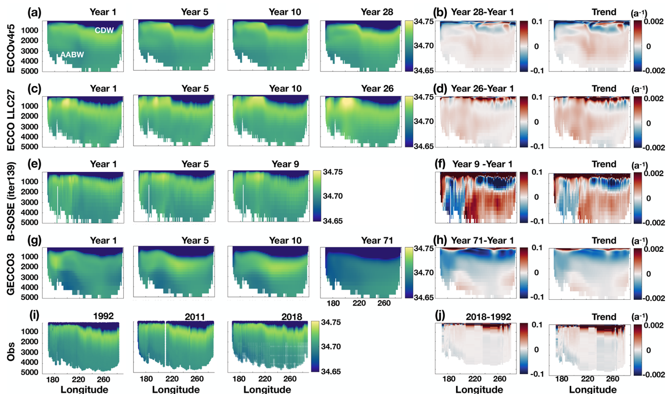
Figure 16. Same as Fig. 12 but for salinity along the S4P section (Fig. 1).
