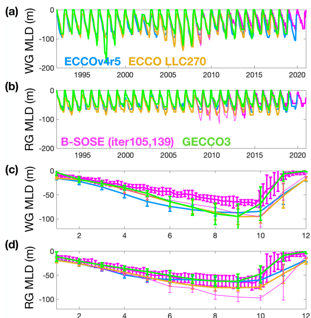
Figure 7. Time series of MLD for the (a) Weddell Gyre and (b) Ross Gyre for locations shown by blue dots in Fig. 1. Climatological MLD seasonal cycle for (c) Weddell Gyre and (d) Ross Gyre. For (c) and (d), error bars represent 1 standard deviation of variability. ECCOv4r5, ECCO LLC270, B-SOSE (iter105), B-SOSE (iter139), and GECCO3 are shown in blue, orange, magenta (thin), magenta (thick), and green, respectively.
