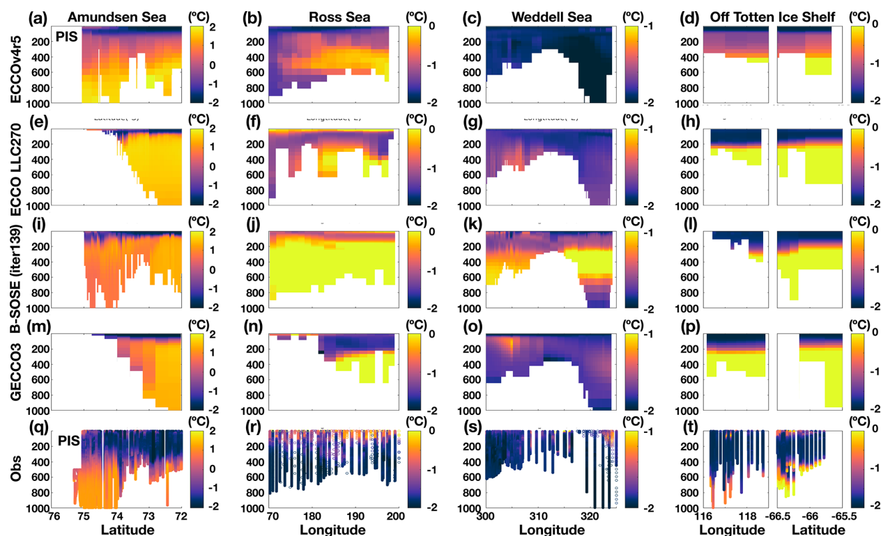
Figure 18. Simulated on-shelf vertical sections of (a–d) ECCOv4r5, (e–h) ECCO LLC270, (i–l) B-SOSE, and (m–p) GECCO3 potential temperature of the final model year for the Amundsen Sea, Ross Sea, and Weddell Sea and off the Totten Ice Shelf. (q–t) The same observed vertical sections of potential temperature compiled from all available years of observations.
