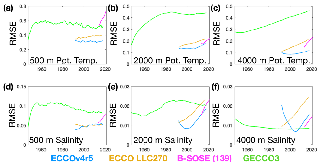
Figure 8. Time series of RMSE of (a, b, c) potential temperature and (d, e, f) salinity at (a, d) 500, (b, e) 2000, and (c, f) 4000 m depth levels. RMSE is calculated by interpolating each ocean state estimate output into a common horizontal grid with 1^\circ resolution. ECCOV4r5, ECCO LLC270, B-SOSE (iter105), B-SOSE (iter139), and GECCO3 are shown in blue, orange, magenta (thin), magenta (thick), and green, respectively.
