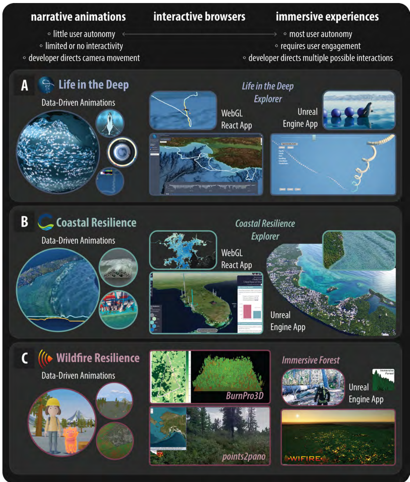
Figure 2: Diagram showing the three types of visualizations (narrative data-driven animation, interactive data exploration tools, and immersive data exploration tools) for each of the three use cases discussed in the paper: (A) Life in the Deep : visualizing impacts on marine ecosystems, (B) Coastal Resilience : visualizing nature-based solutions leveraging the flood protection benefits of coral reefs and mangroves, and (C) Wildfire Resilience : visualizing prescribed fire simulations to inform forest management and prescribed fires.
