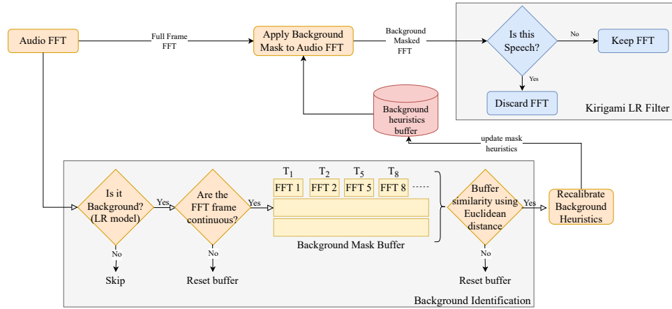
Fig. 7. Flowchart depicts the adaptive background masking process in conjunction with Kirigami’s speech filter. The process involves background detection, buffer comparison, heuristic calculation, and the generation of a background mask to filter out background frequencies. The resulting background-filtered FFT enhances Kirigami’s speech filter for improved accuracy by eliminating background noise.
