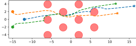
Fig. 1: The trajectories of a 3-agent formation through an obstacle field, where a leader agent (blue) is given a constant control signal directing it straight through the field. Each agent implements safety filtering according to Algorithm 1 and (14) to avoid obstacles while maintaining a formation behavior, according to (30) and (31).
