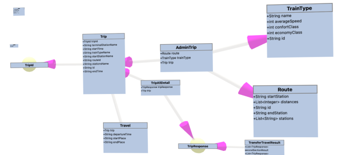
Included Microservices: ts-travel-service, ts-travel2-service, ts-travel-plan-service, ts-common.
