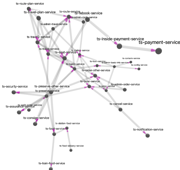
Fig. 3: Service Dependency Graph for Train-ticket benchmark
