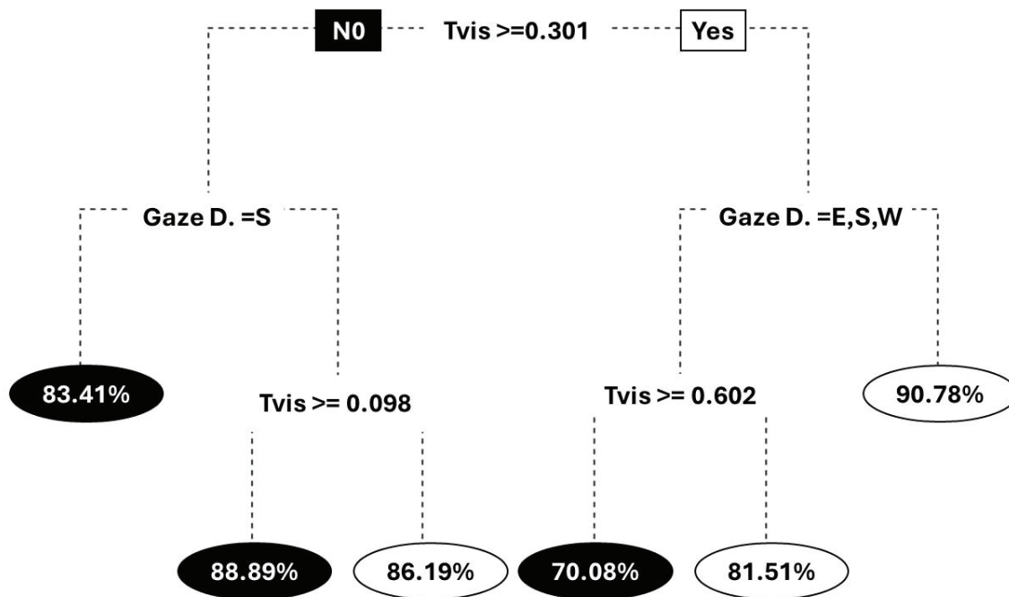
Fig. 5. Using Decision Tree Classification to assess the influence of variables on the level of m_EDI in the second half of the room.
