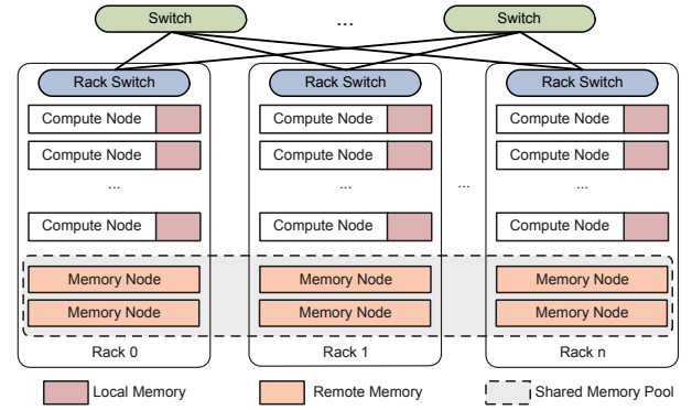
Figure 1: One example of providing a shared memory pool by distributing it across racks.
