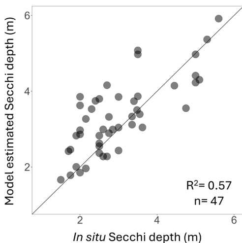
Figure 2. Model performance as observed versus predicted of hold-out data (randomly selected 20% of dataset). Black line is the 1:1 line.
