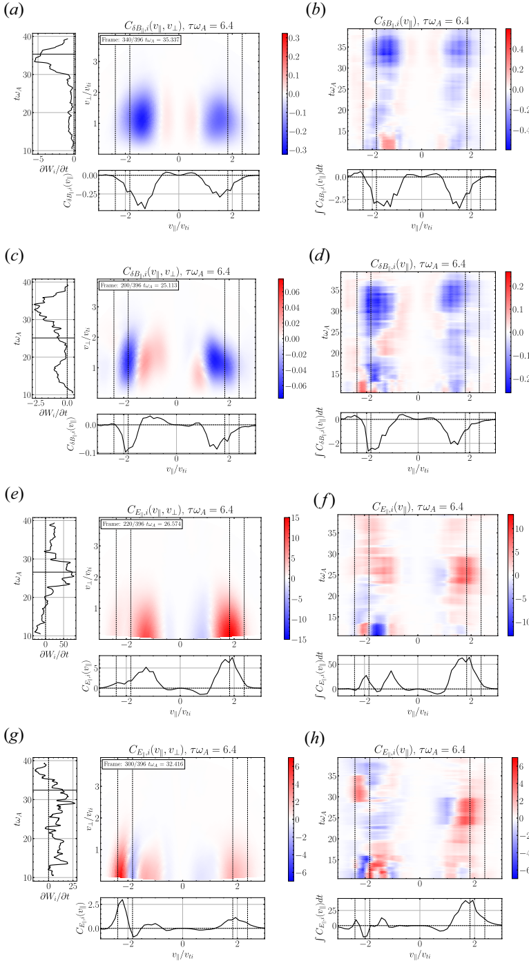
FIGURE 11. Velocity-space signatures of TTD (a–d) and LD (e–h) sampled from AstroGK turbulence simulation with 0.25 \leq k_{\perp}\rho_i \leq 7.75 , T_i/T_e = 1 and \beta_i = 0.3 . The correlation interval is set as \tau\omega_A = 6.4 . (a,c,e,g) Gyrotropic plane ( v_{\parallel}, v_{\perp} ) signatures, and (b,d,f,h) Timestack plots of the v_{\perp} -integrated reduced correlation; both following the layout format of figure 10. The resonant parallel phase velocity ranges are marked by the four vertical dashed lines at v_{\parallel}/v_{ti} = \pm 1.832 and v_{\parallel}/v_{ti} = \pm 2.373 . From top to bottom, data are taken from probe 7 ( 5\pi\rho_i, 3\pi\rho_i, 0 ), probe 15 ( 5\pi\rho_i, 7\pi\rho_i, 0 ), probe 20 ( 4\pi\rho_i, 4\pi\rho_i, -0.125\pi a_0 ) and probe 5 ( \pi\rho_i, 3\pi\rho_i, 0 ), respectively.
