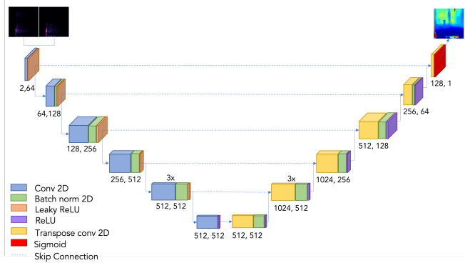
Fig. 8: U-Net Architecture. Input spectrograms are processed to depth maps. Skip-connections used show better performance even though the spatial correspondence between input and output features is not clear.
