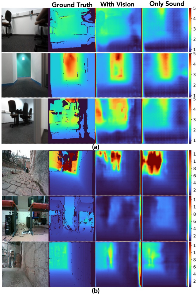
Fig. 6: Test set results when training Beyond Image to Depth on BatVision V1 (a) and BatVision V2 (b), depth in meters. Same hyperparameters as in simulation show well visible general layout and obstacles. Fifth row shows free space between two desks even based on audio-only. Fine structures such as cables are still hard to reconstruct.
