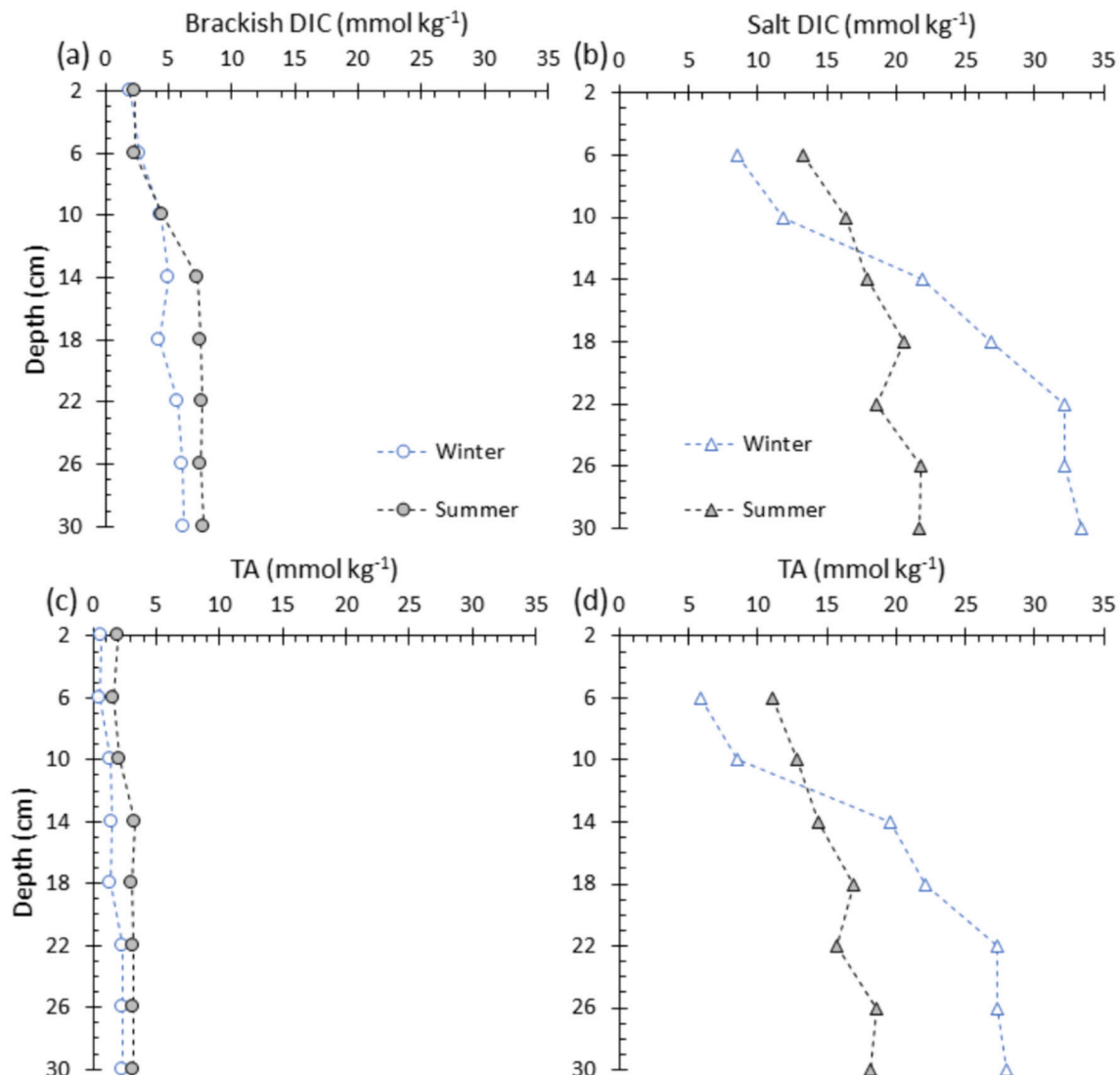
Fig. 3. Infield porewater DIC (a & b) and TA (c & d) concentrations by depth at the brackish marsh (a & c) and salt marsh (b & d).
