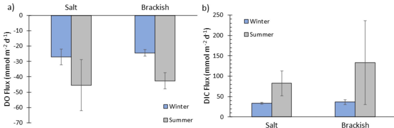
Fig. 4. (a) Aerobic respiration for intact sediment core incubations. (b) Dissolved inorganic carbon production rate for sediment core incubations.
