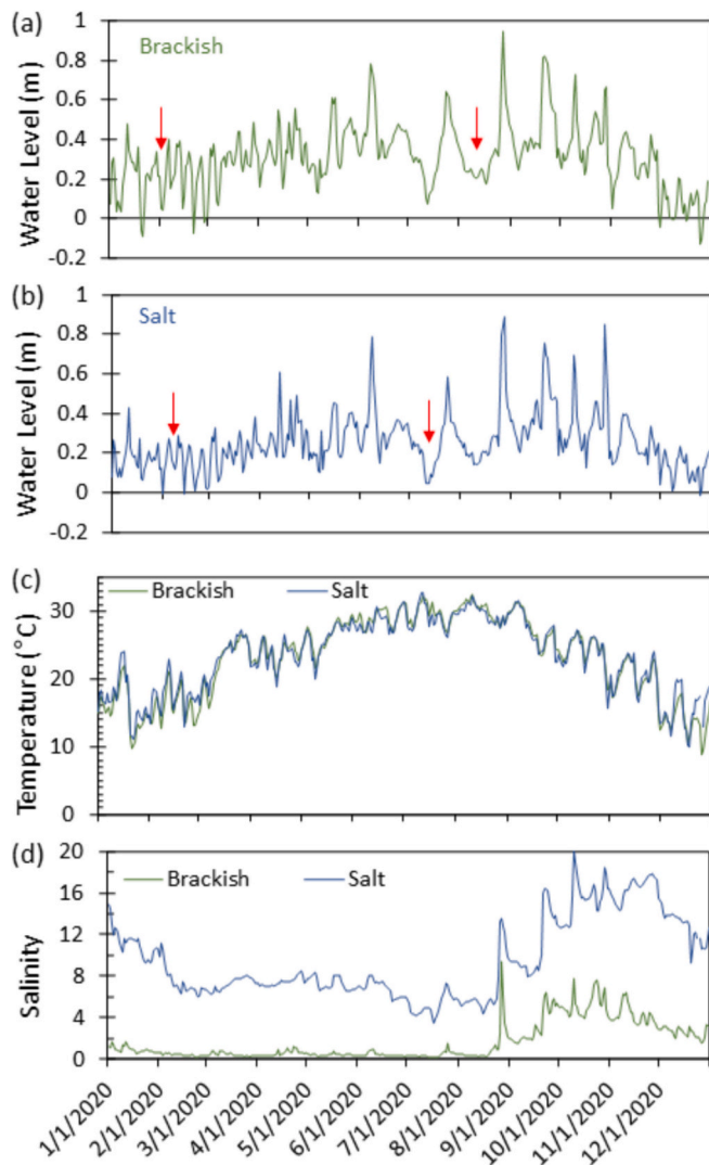
Fig. 2. Surface water level (a, b), temperature (c) and salinity (d) of the brackish and salt marsh sites. Sampling dates are marked with red arrows. Data source: Retrieved from Coastal Information Management System (CIMS) database. http://cims.coastal.louisiana.gov . Accessed 11 November 2023.
