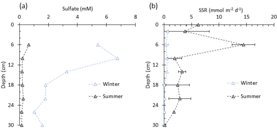
Fig. 6. Water sulfate concentrations (a) and sulfate reduction rates (b) are shown from winter and summer sampling of the salt marsh. Brackish marsh sulfate concentrations were not displayed for clarity between both panels. Note sulfate reducing rates are converted to an areal extent for every 2 cm of the soil core to keep units comparable with other measurements.
