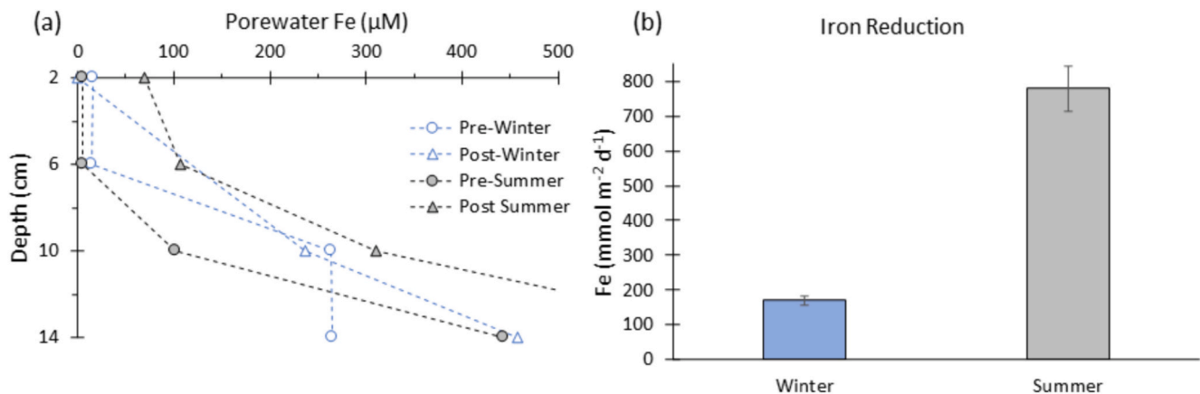
Fig. 5. Iron data for brackish marsh. Porewater iron concentrations for the salt marsh are not shown due to being so small. (a) Porewater concentrations of \text{Fe}^{+2} is shown from pre-incubation samples and post-incubation samples between both seasons. Note 6 cm data is missing in post-winter due sample being container breaking. (b) Iron reduction between seasons at the brackish marsh.
