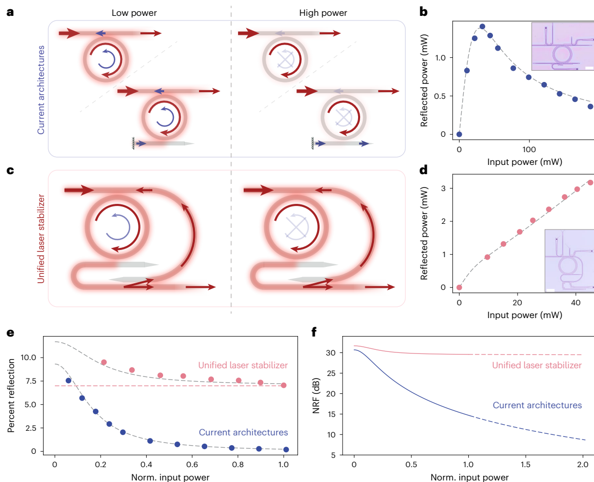
Fig. 3 | High- Q feedback. a , Current self-injection-locking architectures, based on parasitic or intentional back-scattering. Intrinsic ring back-scattering or a reflector are used to generate feedback signal. At low power, this works well, but as the power increases, the backscattered power no longer reaches the laser. b , Theoretical (dashed line) and experimental (data points) back-reflection as a function of input power corresponding to the architectures in a . At low powers, the device is linear and exhibits a constant back-reflection ratio, but as power increases, the nonlinear resonance splitting substantially attenuates the back-reflection. The inset is an image of the device (scale bar, 100 \mu\text{m} ). c , The ULS feedback architecture. Substantial feedback is provided back to the laser regardless of input power. d , Theoretical (dashed line) and experimental (data points) back-reflection as a function of input power corresponding to the
