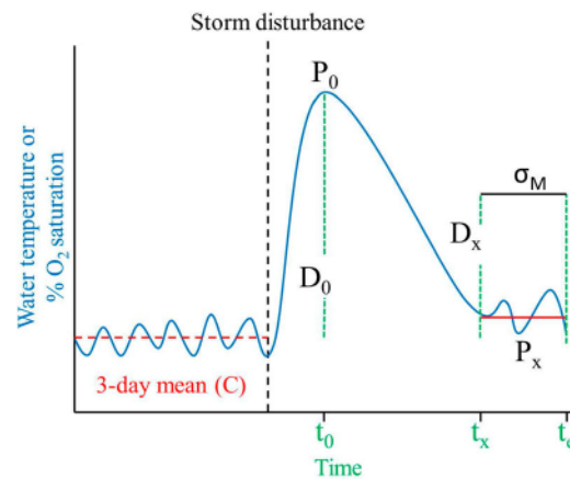
Figure 1. Schematic depicting how to apply equations 3 and 4 to calculate resistance and resilience indices of lake water temperature and percent oxygen saturation (y-axis, blue line) responding to a storm disturbance (vertical black dashed line), and peaking ( P_0 ) at time t_0 and recovering ( P_x , horizontal red solid line) between time t_x and t_e . Vertical green dashed lines represent times (x-axis) at which D_0 and D_x are calculated. Resistance (RS) is therefore the difference between the absolute peak displacement in water temperature or percent oxygen saturation and their respective 3-day mean control conditions (C, horizontal red dashed line), or |D_0| = |C - P_0| . Resilience (RL) is then calculated by taking the absolute difference between C and the mean value of P_x averaged over a 72 h window with the lowest standard error ( \sigma_M , horizontal black solid line) in water temperature or percent oxygen saturation, or |D_x| = |C - P_x| . Both resistance and resilience indices range between -1 and 1 , where a 1 indicates total resistance and resilience. A resistance value of 0 represents times when water temperature or oxygen saturation conditions were displaced by 100\% , either increasing or decreasing relative to antecedent conditions. Therefore, a resilience value of 0 indicates water temperature or oxygen saturation remained at peak displacement levels, or there was 0\% recovery. Thus, negative values of resistance represent times of more than 100\% displacement, while negative values of resilience represent times when water temperature or oxygen saturation continued to drift further from peak displacement levels, or overcompensated in their recovery by overshooting the 3-day mean antecedent control conditions.
