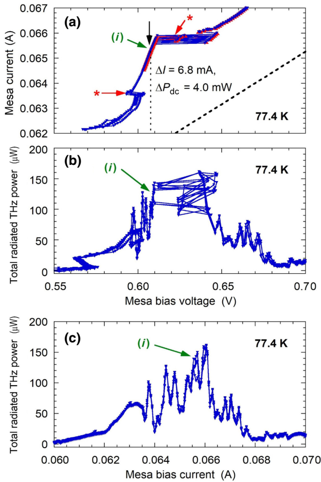
FIG. 8. p = 0.16 , N = 596 , 300 \times 180 \times 0.92 \mu\text{m}^3 ( l \times w \times t ). (a) Plot of the unusual voltage jumps (labeled with red asterisks) seen for the 300 \times 180 \times 0.92 \mu\text{m}^3 mesa at a cryogenic bath temperature of 77.4 K. Blue inverted triangles are current-voltage data collected while sweeping the current downwards, while red triangles are current upsweep data. Ten sets of data are plotted sweeping in each direction. Green label (i) indicates the current-voltage point at which the FTIR spectrum shown in Fig. 4(d) is measured. Diagonal dashed black line indicates the tangent to the current-voltage curve, corresponding to the estimated low-bias resistance of the mesa. Vertical dotted line indicates the estimated current-voltage anomaly associated with this terahertz mode. (b) Total integrated terahertz emission power measured while sweeping the current downwards, plotted as a function of bias voltage over the same range as for (a). Data for five downward current sweeps are shown. (c) Terahertz emission power measured while sweeping the current downwards, plotted as a function of bias current over approximately the equivalent biasing range. Owing to the excellent reproducibility of our results with respect to bias current, the five data sets plotted are almost indistinguishable.
