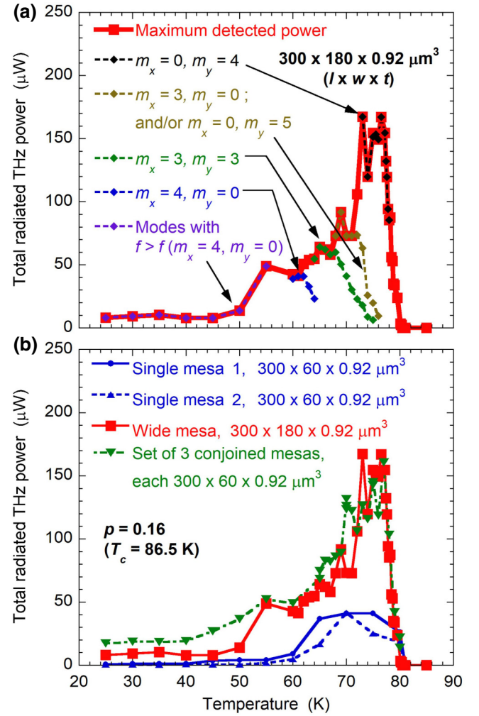
FIG. 7. (a) p = 0.16 , N = 596 , 300 \times 180 \times 0.92 \mu\text{m}^3 ( l \times w \times t ). Maximum total radiated terahertz power that could be generated by the 300 \times 180 \times 0.92 \mu\text{m}^3 mesa at each temperature (red curve, squares). Where one or more modes could be clearly identified at each temperature, the emission power from each of these is plotted also (diamonds). (b) Maximum total radiated terahertz power plotted against temperature, for all four devices fabricated on this chip. Blue curves (circles and triangles) show emission for the two individual 300 \times 60 \times 0.92 \mu\text{m}^3 mesas. Red curve (squares) shows emission for 300 \times 180 \times 0.92 \mu\text{m}^3 mesa, while the green dashed curve (inverted triangles) shows emission for the set of three conjoined 300 \times 60 \times 0.92 \mu\text{m}^3 mesas.
