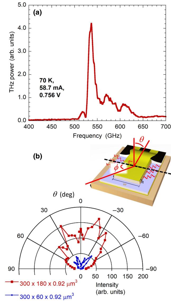
FIG. 6. p = 0.16 , N = 596 , 300 \times 180 \times 0.92 \mu\text{m}^3 ( l \times w \times t ). (a) Terahertz emission spectrum as measured by FTIR from 300 \times 180 \times 0.92 \mu\text{m}^3 mesa at a cryogenic bath temperature of 70 K and a bias current of 58.7 mA. This spectrum is very broad and multi-peaked, indicating that synchronization of the junctions is quite unstable under these conditions. The most probable modes being excited are ( n = 0 , m_x = 3 , m_y = 0 ) and/or ( n = 0 , m_x = 0 , m_y = 5 ). (b) Angle dependence of the terahertz emission for this device as measured under the same operating conditions as in (a) as a function of polar angle \theta , i.e., when rotating about the long axis of the mesa. For comparison, data from one of the 300 \times 60 \times 0.92 \mu\text{m}^3 mesas on the same chip are plotted, also operating at 70 K, in the ( n = 0 , m_x = 1 , m_y = 0 ) and/or ( n = 0 , m_x = 0 , m_y = 5 ) mode. Diagram shows the definition of the polar angle \theta and azimuthal angle \phi as referred to in this work.
