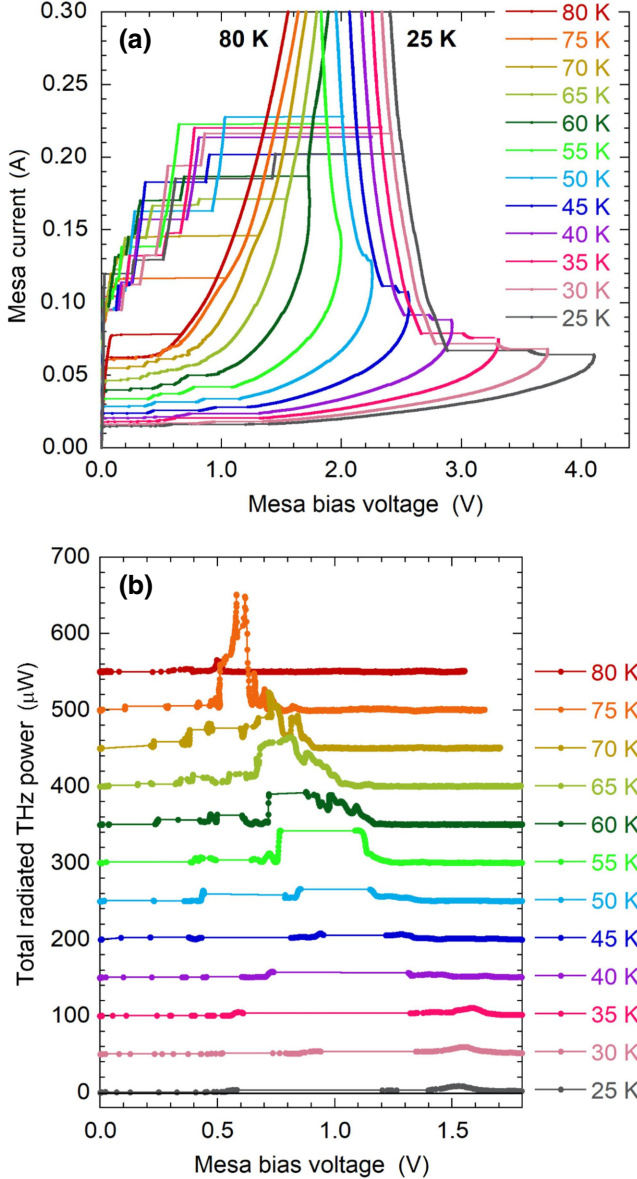
FIG. 4. p = 0.16 , N = 596 , 300 \times 180 \times 0.92 \mu\text{m}^3 ( l \times w \times t ). (a) Current-voltage characteristics for 300 \times 180 \times 0.92 \mu\text{m}^3 mesa at a range of cryogenic bath temperatures, showing hysteretic switching of stacked IJJs. For this device, terahertz emission always occurs on the downward sweep, and only in the low-current bias regime (i.e., not in the back-bending regions). (b) Total integrated radiated terahertz power plotted against voltage for the same device. For clarity, successive curves are offset by 50 \mu\text{W} , and only data recorded on the current downswing are shown. Note also that the voltage scale differs from that shown in (a). (No terahertz emission occurs at mesa bias voltages exceeding 1.8 V for this device.)
