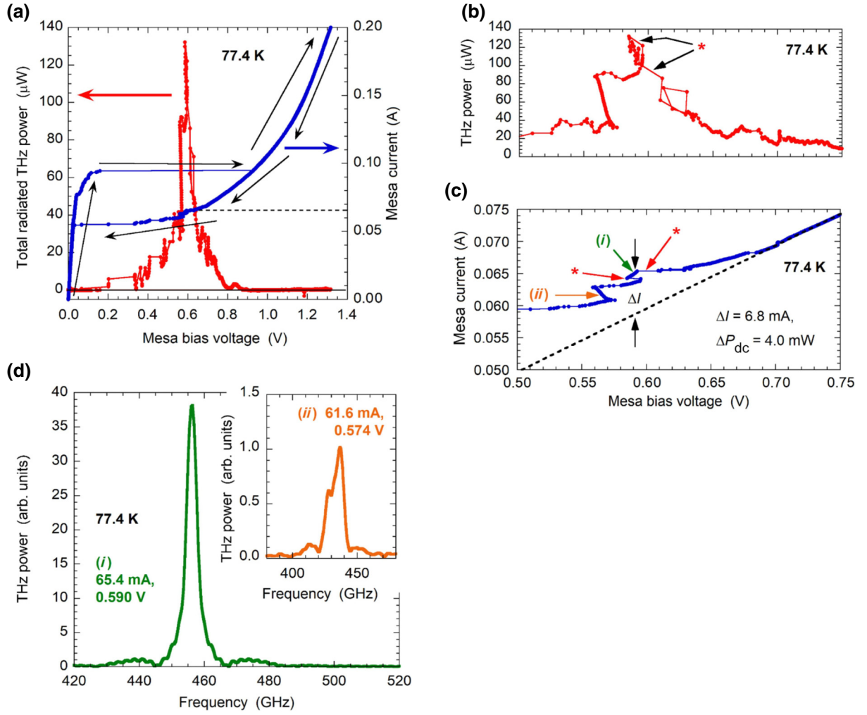
FIG. 3. p = 0.16 , N = 596 , 300 \times 180 \times 0.92 \mu\text{m}^3 ( l \times w \times t ). (a) Mesa bias current for 300 \times 180 \times 0.92 \mu\text{m}^3 mesa and total integrated radiated terahertz power, plotted against mesa bias voltage, at a bath temperature of 77.4 K. Black arrows indicate the direction in which current is swept. (b) Detail of the terahertz power emission plotted in (a), close to the emission mode. (c) Detail of the I - V characteristic plotted in (a), over the same range of voltages as in (b). The dashed black line is a straight line fit through the origin assuming a constant device resistance, allowing us to estimate the excess current and power drawn by the resonant terahertz mode. The voltage steps labeled with the arrows and red asterisks are discussed in the text. (d) Main image shows FTIR spectrum for terahertz emission from the same device, collected close to maximum emission power at this temperature, labeled as point (i) in (c). Bias current of 65.4 mA is indicated by the dotted horizontal line in (a) above. As-measured FWHM linewidth is limited by the 2.25 GHz resolution of the spectrometer. Inset shows emission spectrum measured at 61.6 mA on the reentrant section of the current-voltage curve at the same temperature, labeled as point (ii) in (c). The emission spectrum is much broader and multimodal, while emission power is much weaker than in the main plot. (Please note the different scales for the power and frequency axes in the inset.)
