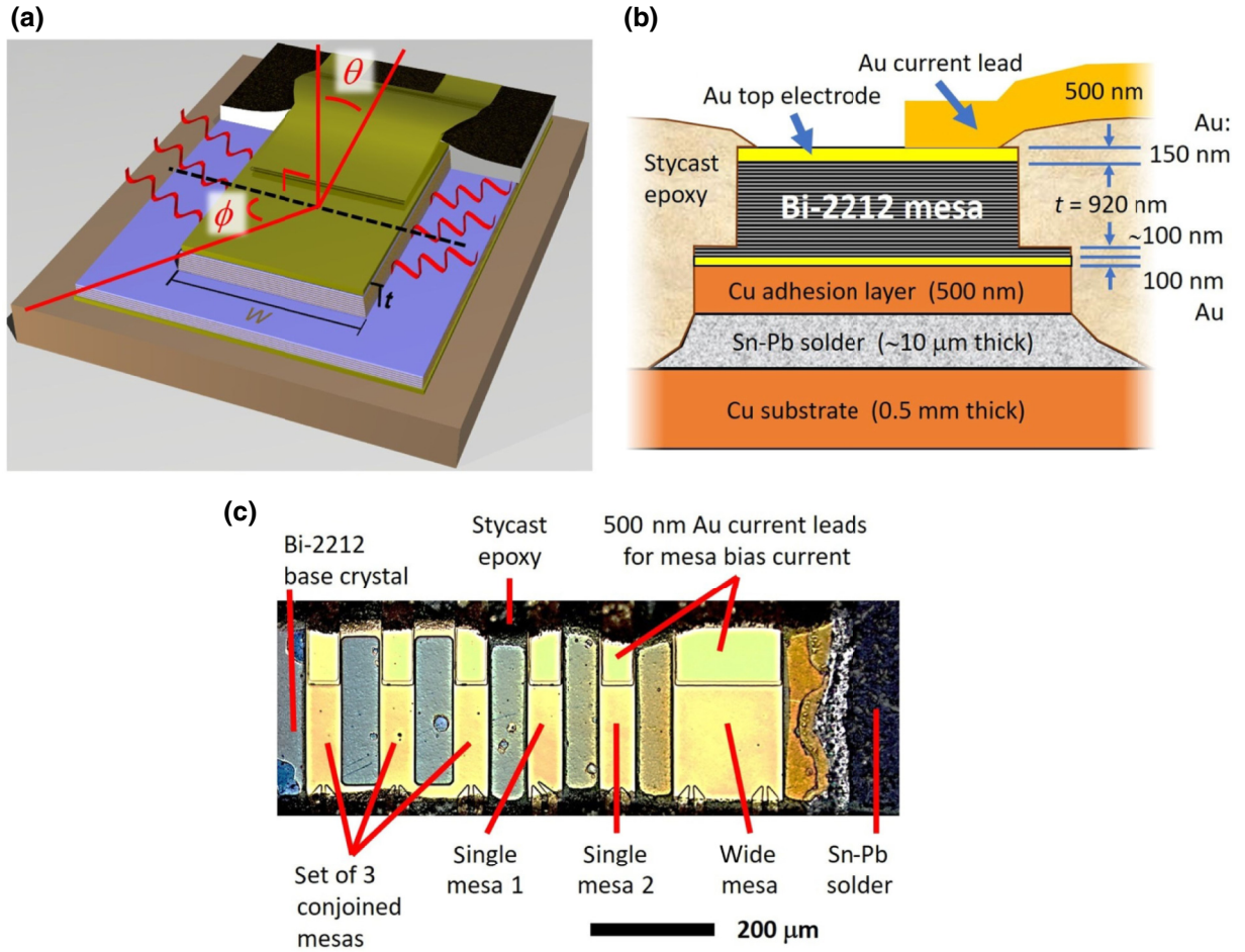
FIG. 1. (a) Schematic showing the geometry of a typical Bi-2212 mesa designed for coherent terahertz emission, after Ref. [28], with the IJJ stack having width w and total thickness t . For clarity, vertical scale is shown greatly exaggerated with respect to lateral scale. Red wavy lines are a schematic indication of the direction of greatest far-field radiated terahertz intensity, and the indicated wavelength is not drawn to scale. Actual wavelength of the emitted radiation is approximately 600 \mu\text{m} , which is twice the mesa length. Polar angle \theta and azimuthal angle \phi as defined in this work are indicated. Current is supplied to the stacked IJJs via the gold top electrode and sunk via the base crystal. Any dc power dissipated in the device is also heat sunk via the base crystal. (b) Schematic showing vertical cross section of the devices studied in this work, including the metal thin films deposited on the top and bottom surfaces of the Bi-2212 crystal. For clarity, vertical distances are shown greatly exaggerated and not to scale. (c) Optical micrograph of the four devices studied in this work, with important parts of microchip labeled. Note that the Bi-2212 base crystal is so thin that it is almost transparent, and the metal adhesion layers underneath can be seen. The gold tracks at the top end of the mesas are for supplying bias current to the mesas themselves, while those at the bottom end are current leads for future installation of NiCr thin-film heaters, intended for studying the effects of localized heating of the mesas. Note that the metal tracks deposited on the epoxy appear slightly out of focus in this image, since the epoxy surface lies a few microns above the plane of the top of the mesas.
