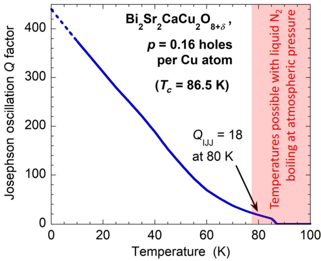
FIG. 2. Q_{IJJ}(T) as calculated using Eq. (5) for optimally doped Bi-2212, with p = 0.16 holes per Cu. The experimental data sets obtained from Ref. [31] only extended as low as 10 K, so data below this temperature are a linear extrapolation (shown dotted).
