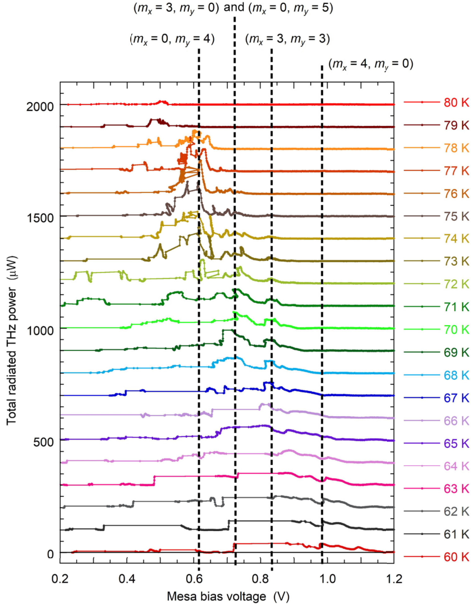
FIG. 5. p = 0.16 , N = 596 , 300 \times 180 \times 0.92 \mu\text{m}^3 ( l \times w \times t ). Total integrated radiated terahertz power for 300 \times 180 \times 0.92 \mu\text{m}^3 mesa plotted against voltage. These data are for the same device as shown in Fig. 4, but at more closely spaced temperatures. For clarity, successive curves are offset by 100 \mu\text{W} . Vertical dashed lines show the four strongest modes of terahertz emission, labeled with their most probable indices for (m_x, m_y) , assuming n = 0 .
