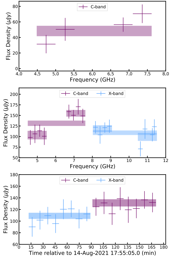
Figure C1. Top: the 11.2 day VLA C-band observation, broken up into four 256 MHz bins (error bars indicate the 1\sigma flux density and width of the frequency bin). The shaded region indicates the flux density of the full C-band bandwidth at 1\sigma , with the width of the shaded region indicating the bandwidth. Middle: the 19.0 day VLA C-band (purple points) and X-band (blue points) observations, broken up into 16 128 MHz bins (eight bins per band; error bars indicate the 1\sigma flux density and width of the frequency bin). The shaded regions indicate the flux density of the full C-band (purple) and X-band (blue) bandwidth, at 1\sigma , as well as the flux density of the lower and upper sidebands, the widths of the shaded regions indicating the bandwidth. Bottom: the 19.0 day VLA C-band (purple points) and X-band (blue points) observations, broken up into 16 \sim 510 s time bins (eight bins per band; error bars indicate the 1\sigma flux density and width of the time bin). The shaded regions indicate the flux density of the full C-band (purple) and X-band (blue) bandwidth at 1\sigma , with the widths of the shaded regions indicating the temporal coverage of the observation at that band.
