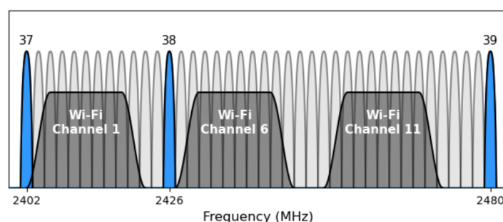
Figure 1. BLE and WiFi channel spectrum (revise the diagram).
