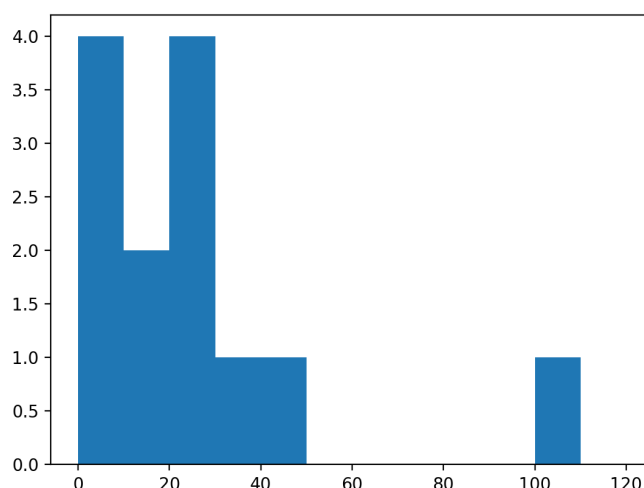
Figure 18. Histogram of the difference between the estimated DOA and actual direction of the BLE beacon.
