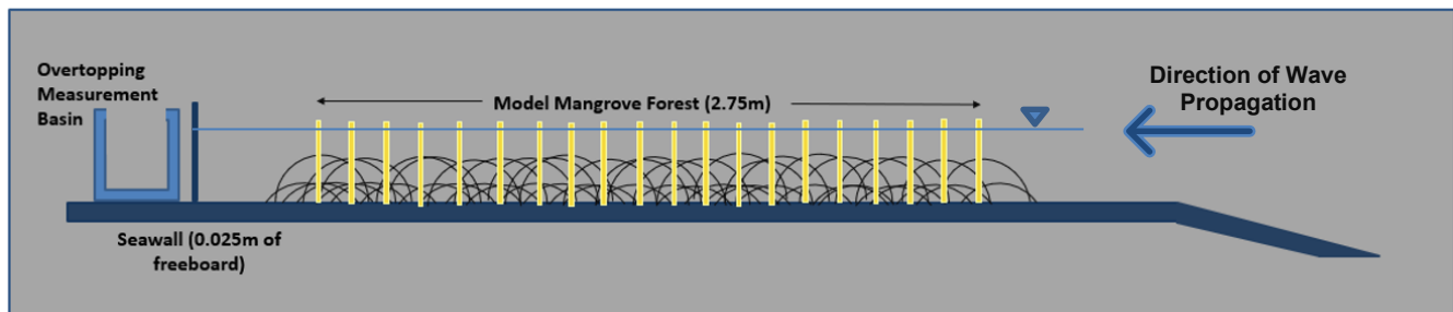
Figure 3. Profile diagram of experiments (not to scale).
