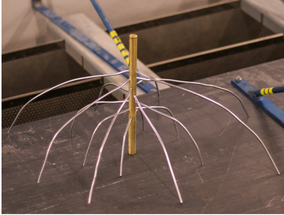
Figure 1. Photograph of a 1:8 scale model mangrove used in USNA experiments made of brass rod of 1.5cm diameter and 6-gauge galvanized steel wire.
