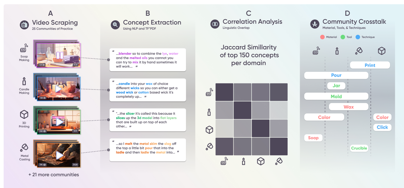
Figure 1: A) Metadata and transcripts are collected from 1.8k video tutorials across 25 creative Communities of Practice (CoPs); B) Part-of-speech tagging and TF*PDF ranking on tutorial transcripts is used to extract and highlight the most relevant concepts for each community; C) A similarity matrix with agglomerative hierarchical clustering is used to draw insight on semantic overlaps between communities; D) Using a LLM, concepts are tagged as "Material", "Tool", and "Technique", providing a more detailed look at the interplay between adjacent and disparate communities.
