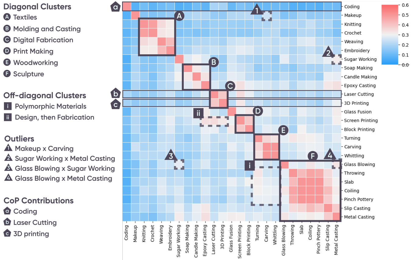
Figure 2: CoP Similarity Cluster Heatmap. A visualization of the shared concepts between 25 CoPs. The Jaccard index is used to computer similarity between CoP A and CoP B. UPGMA (Unweighted Pair Group Method with Arithmetic Mean) is used as the linkage method to perform unsupervised agglomerative clustering for hierarchical structure discovery. CoP rows and columns are arranged such that practices that share more concepts with each other are placed closer together.
