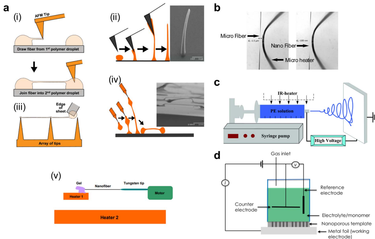
Fig. 15 Different methods to make nanofiber. (a) Sharp tip drawing. (i) Draw fiber from 1 st polymer droplet. Reproduced with permission. 246 Copyright, 2004, American Chemical Society – NL. (ii) AFM tip joining two PMMA droplets to make nanofiber. Reproduced with permission. 247 Copyright, 2006, Institute of Electrical and Electronics Engineers . (iii) Joining two sharp tips with the edge of a sheet. Reproduced with permission. 246 Copyright, 2004, American Chemical Society – NL. (iv) Micro-pipette probe-based drawing technique. Reproduced with permission. 247 Copyright, 2006, Institute of Electrical and Electronics Engineers . (v) Polyethylene drawing using a sharp tungsten tip on a heating stage. Reproduced with permission. 98 Copyright, 2010, Nature Nanotechnology . (b) Transient heat stretching (left) before heating and microfiber, (right) after heating and nanofiber. Reproduced with permission. 138 Copyright, 2018, Nature Communications . (c) Schematic of electrospinning setup with an embedded IR heater. Reproduced with permission. 113 Copyright, 2015, Royal Society of Chemistry – Nanoscale . (d) Schematic of nanoscale templating technique. Reproduced with permission. 109 Copyright, 2014, Nature Nanotechnology .
