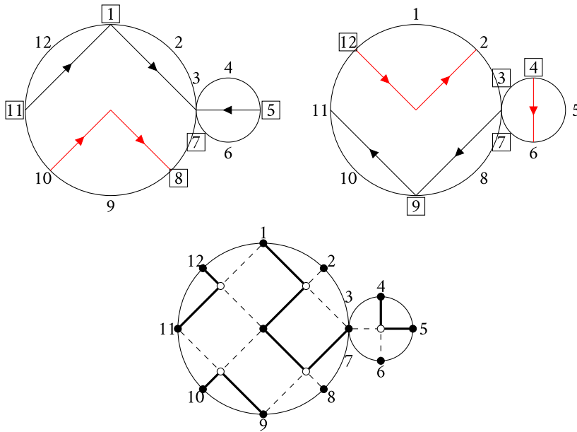
Figure 17: The map \psi in the proof of Theorem 5.5 with \xi = (1, 10|2, 9|3, 12|4, 6|5, 7|8, 11) , I = \{1, 5, 7, 8, 11\} , J = \{3, 4, 7, 9, 12\} . Top left: F_I \cup \tilde{F}_I ; top right: F_J \cup \tilde{F}_J ; bottom: the selection A in N(\xi) with edges in \Gamma colored in black and edges in \Gamma^\vee colored in red.
