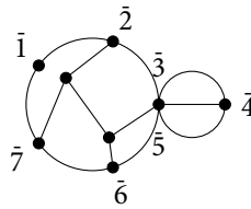
Figure 2: An example of a cactus network for \zeta = (\bar{1}|\bar{2}|\bar{3}, \bar{5}|\bar{4}|\bar{6}|\bar{7}) .
