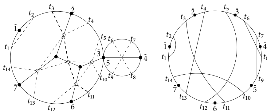
Figure 3: A cactus network \Gamma with its medial graph G(\Gamma) (left) and medial pairing \tau(\Gamma) = \{(1, 2), (3, 11), (4, 13), (5, 12), (6, 8), (7, 9), (10, 14)\} (right).
