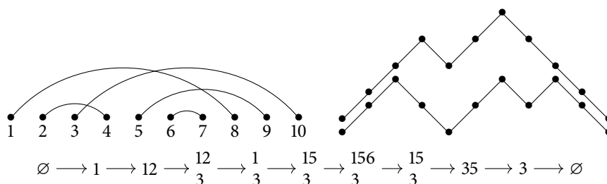
Figure 8: A bijection between \mathcal{TC}_n and \mathcal{C}_n^{(2)} by Chen et al. [CDD + 07], with the sequence of standard Young tableaux T_0, T_1, \dots, T_{2n} shown below.
