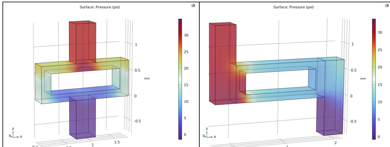
Figure 2 COMSOL CFD Simulation showing the pressure distribution on the membrane for the “Perpendicular Control” Valve. Left: Pressure distribution on the membrane of the naive design under actuation, highlighting unevenly high stresses at the membrane center, potentially leading to rupture or mechanical failure. Right: Pressure distribution on an optimized design, demonstrating how stresses are shifted away from the membrane’s center—the weakest part—toward more structurally robust regions.
