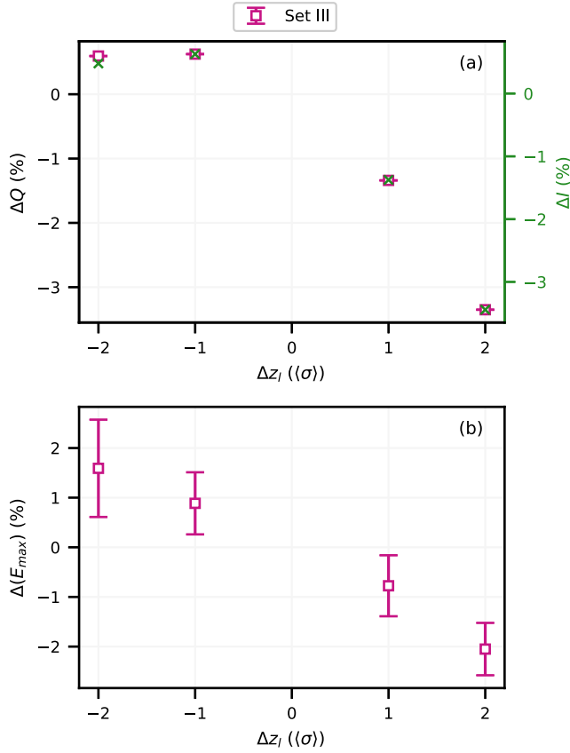
FIG. 9. Simulated ramp position fluctuations in a tailored plasma target after 1.2 mm. Deviation of (a) injected charge and (b) maximum electron beam energy from the baseline. \Delta z_l = 0 corresponds to the middle of the ramp aligned with the vacuum laser focus; positive \Delta z_l corresponds to a vacuum laser focus after the ramp. The green crosses in (a) depict the measured laser intensity deviations after 0.4 mm propagation.
