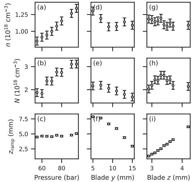
FIG. 3. The left column shows the response of (a) plateau density, (b) peak density, and (c) ramp position as a function of backing pressure. (d)–(f) and (g)–(i) show the same parameters for blade height and blade coverage, respectively. Each point is the average of three to five shots and the error bars represent the shot-to-shot fluctuations ( \pm 1\sigma ) discussed in Sec. II C. For the pressure scan, y = 6.5 mm and z = 3.2 mm. For the blade y scan, P = 100 bar and z = 3.5 mm.
