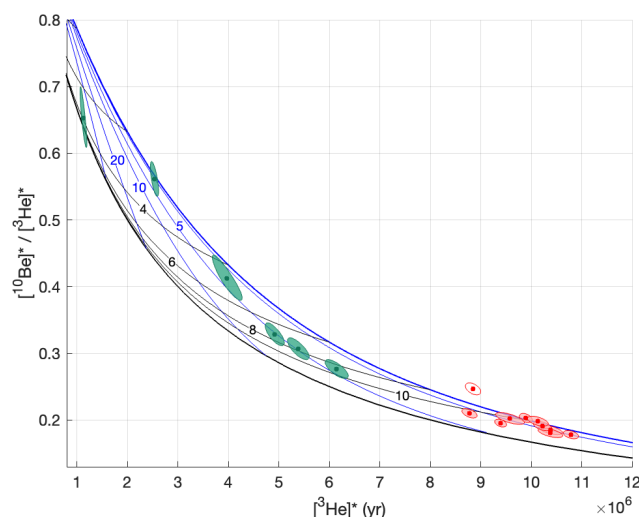
Figure 2. A ^{10}\text{Be} - ^3\text{He} two-nuclide diagram. Red data points show measurements from this study, green data points are from Balter-Kennedy et al. (2023), and each shaded ellipse represents the 68 % confidence interval in the measured nuclide concentrations. The thick blue line is the simple exposure line, and the thin blue lines are lines of constant erosion ( \text{m Myr}^{-1} ). The thick black line is the steady-erosion line, and the thin black lines are constant-age lines ( \text{Myr} ). * signifies nuclide concentrations normalized to site-specific production rate for comparison across sampling locations.
