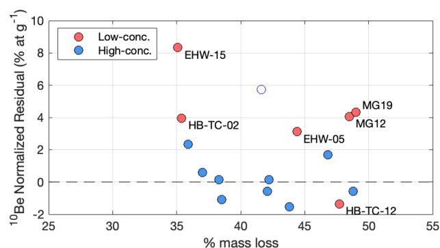
Figure 5. Comparison of mass lost during HF etching with normalized residuals between measured ^{10}\text{Be} concentrations in samples and expected concentrations. For the high-concentration samples (blue), the expected values are given by the dashed line in Fig. 1. For the low-concentration samples (red), the expected values are given by the linear regression in Fig. 4. The white dot represents the outlier as discussed in Fig. 1.
