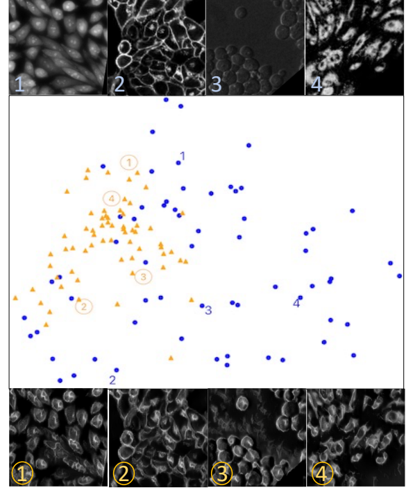
Fig. 6: VGG feature embedding for original (top, blue) and stylized images (bottom, orange).
