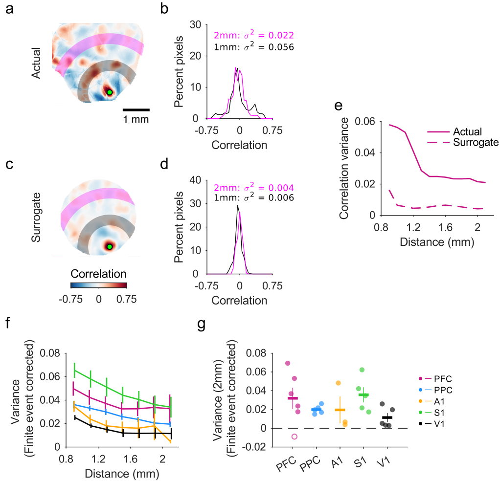
Fig. S5. Assessment of long-range correlations in spontaneous activity through correlation variance. a,b. Correlation strength was measured by computing the variance of the distribution of correlation values within bins of increasing distance from the seed point. Correlation pattern with distance bins is shown in (a) and the distribution of correlation values within these bins in (b). Regions of strong correlations have both strongly positive and strongly negative values within the bin, leading to a high variance (e.g. near a seed point, black line). Weak correlations (e.g. further from a seed point, magenta) will be closer to zero and exhibit reduced variance. c,d. Same as for (a,b) but for a surrogate correlation pattern computed for an equal number of patterns as in (a) (see Methods). Distributions of correlation values are narrow, and vary little with distance. e. Plot of correlation variance as a function of distance from the seed point for the 'actual' correlation pattern (a) and the surrogate pattern (c). The variance of the surrogate was subtracted from that of the actual correlation pattern to control for the finite number of events recorded during imaging. f. Variance of correlations as a function of distance for all cortical areas after subtracting surrogate values. Data shown as mean \pm SEM across all FOVs within an area. g. Correlation variance 2 mm from seed points is similar across cortical areas (KW: H(4) = 5.34 , p = 0.254 ). Filled circles (24 of 25 FOVs) indicate experiments with statistically significant correlations at 2 mm relative to surrogate controls (dashed line at zero).
