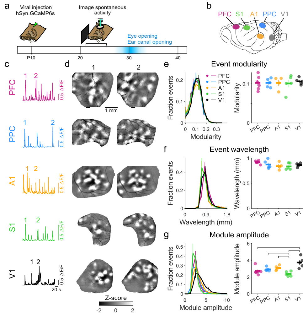
Figure 1: Spontaneous activity is highly modular in early development across diverse cortical areas. a. Experimental schematic. Spontaneous activity is imaged at P21-24, 7-14 days prior to eye-opening and ear canal opening. b. Activity was imaged in primary somatosensory (S1), auditory (A1), and visual (V1) cortices, and in the association areas prefrontal cortex (PFC) and posterior parietal cortex (PPC). c. Time course of spontaneous activity (mean activity across ROI) in each brain area imaged in independent experiments. d. Individual spontaneous events (times indicated in (c)) show highly modular activity in all areas. e. The modularity of spontaneous events does not vary across cortical areas. For panels (e-g): Left plot shows distribution across all events, Right plot shows median of distribution for each animal (dots) and mean across animals (horizontal bar). f. The wavelength of activity for spontaneous events is similar across events from different areas. g. Module amplitude (active module vs adjacent cortex) is generally similar across areas, with significantly lower amplitude in S1 and higher amplitude in V1. Significant post-hoc pairwise comparisons indicated by horizontal lines. Error bars: \pm SEM.
