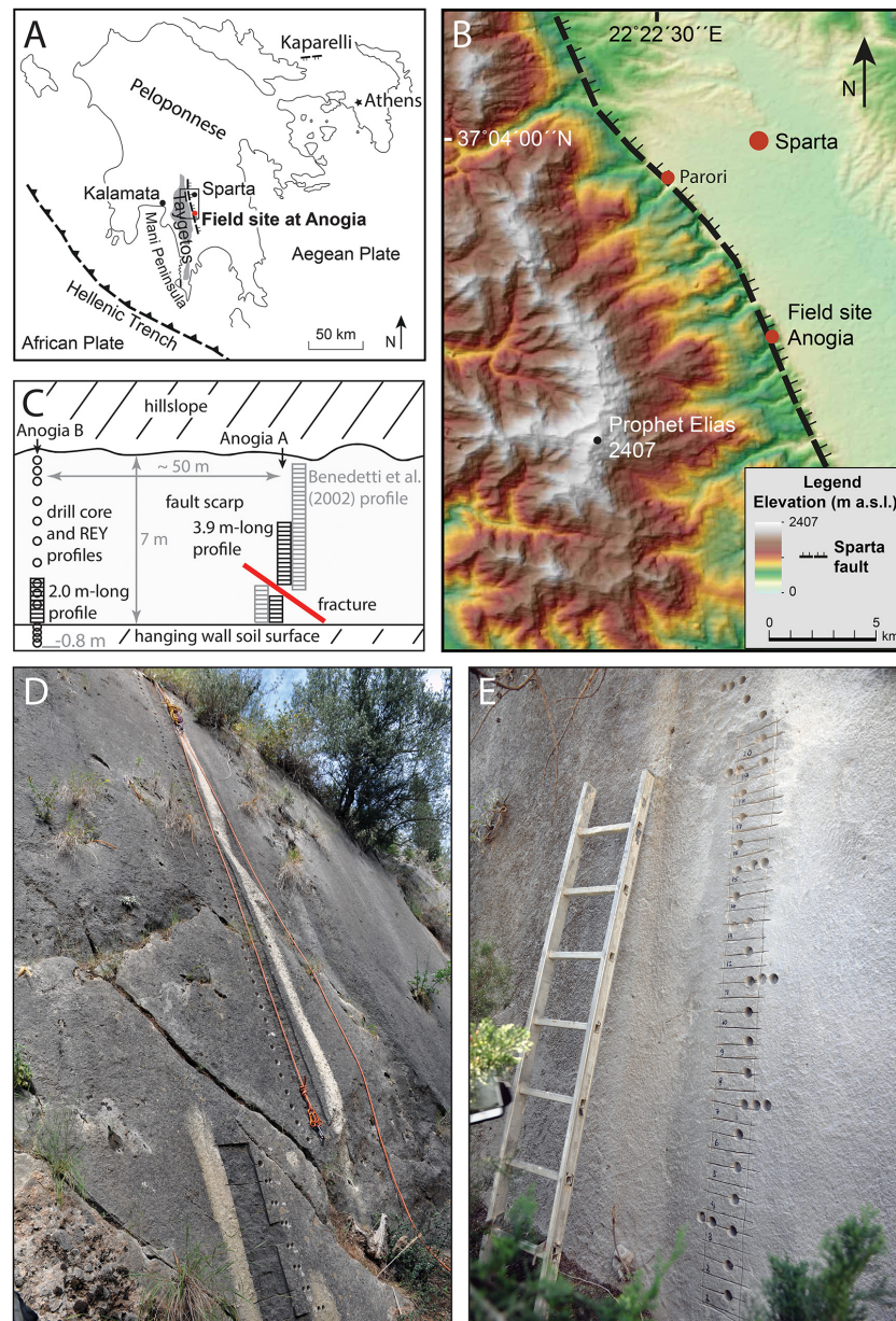
Figure 1. Study site. (a) The study site location in the Peloponnese, Greece. Key tectonic features are shown. The box indicates the location of panel (b). (b) The location of the Sparta Fault, separating the Taygetos mountains from the Sparta basin. The location of the Anogia field site used both in this study and in Benedetti et al. (2002) is shown. Benedetti et al. (2002) located a second sampling transect at Parori (also shown). The digital elevation model has a 24 m resolution and is derived from ASTER GDEM (GDEM2), which is a product of NASA and METI (Japan). (c) Schematic diagram of the Sparta Fault scarp at Anogia, showing the locations of our vertical ^{36}\text{Cl} and REE-Y sampling transects and the ^{36}\text{Cl} sampling transect of Benedetti et al. (2002). (d) Photograph showing the location of the Anogia A profile prior to sampling. The existing sample scar is from Benedetti et al. (2002). (e) Photograph showing the location of our REE-Y and drill core profiles after sampling and the Anogia B profile before slab sampling.
