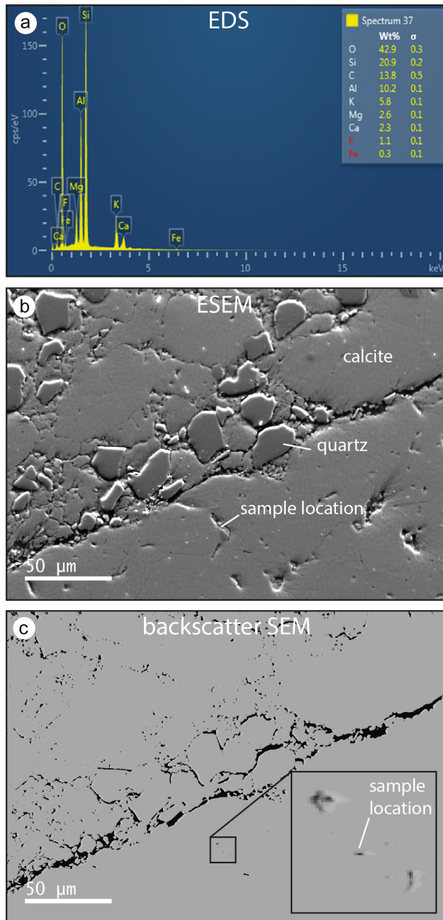
Figure 8. Energy-dispersive X-ray spectroscopy (EDS) elemental abundances and environmental scanning electron microscope (ESEM) and backscatter SEM imagery of a thin section of fault breccia comprising the Sparta Fault scarp surface at 1.1 m above the hanging wall. (a) Element abundances in a pore, the location of which is shown in panels (b) and (c) . Si, Al, and K are abundant relative to Ca, which indicates that clay, e.g. illite, is lining the pore. (b) Quartz is an abundant constituent of the thin-section matrix. (c) Porosity, shown in black; note its spatial association with quartz. The location of the sample used in panel (a) is in a small pore, shown in the inset.
