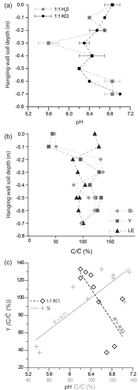
Figure 12. Hanging-wall soil chemistry, adjacent to the Sparta Fault scarp at Anogia. (a) Soil pH along a vertical profile measured from soil mixed with distilled H 2 O and 1M KCl. Uncertainty ranges show the \leq 0.5 resolution of the indicator strips. (b) Concentrations of Si, Y, and elements too light to be measured using hand-held XRF (LE, including C) along the vertical soil profile. Each element has been normalized through division by its mean concentration through the soil. (c) Y concentrations plotted against pH (measured from 1 : 1 KCl) and Si concentration at each measured depth interval beneath the soil surface.
