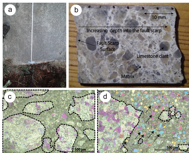
Figure 6. The heterogeneous fault breccia that comprises the Sparta Fault scarp surface. (a) The Sparta Fault scarp surface appears smooth and homogenous, as illustrated by this photograph of the scarp base at Anogia (the upper half of the dug trench in the foreground). (b) Fault breccia is revealed in a cut drill core, where clasts of host limestone are cemented in a fine matrix. (c) A photomicrograph shows limestone clasts (dotted outlines) comprising about 60 % of the thin-section area. (d) A photomicrograph shows fine matrix comprising about 60 % of the thin-section area. Arrows indicate quartz.
