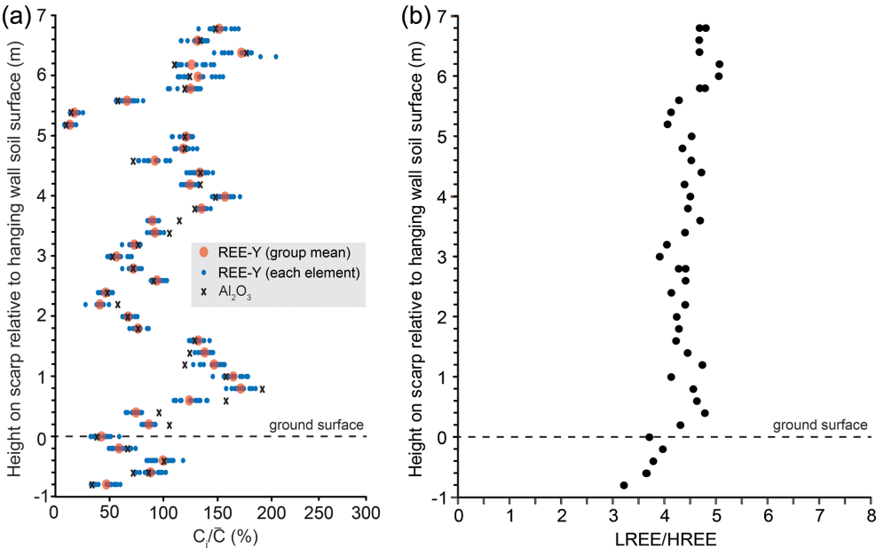
Figure 10. Vertical distribution of REE-Y elements on the Sparta Fault (Anogia B profile). (a) REE-Y concentrations. Mean values for all REE-Y elements at each sample point are shown in red dots, whereas individual REE-Y elements are shown in blue dots. The concentration of each element ( C_i ) is normalized to its mean concentration through the profile ( C_i/\bar{C} ). Concentrations of Al_2O_3 are shown for reference. (b) LREE : HREE ratio. There are two measurements at -0.6 m.
