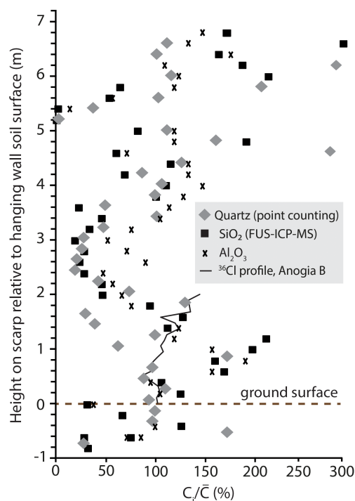
Figure 7. Concentrations of \text{Al}_2\text{O}_3 and \text{SiO}_2 , and quartz abundances from point counting, along a vertical profile, Sparta Fault scarp, Anogia. The concentration of each element ( C_i ) is normalized to its mean concentration through the profile ( C_i/\bar{C} ). The ^{36}\text{Cl} concentration profile is shown for reference.
