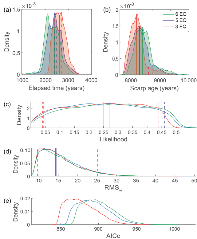
Figure 4. Statistical plots for Markov chain Monte Carlo (MCMC) modelling. Results are shown for three, five, and six model earthquakes. Solid vertical lines indicate the median of each distribution, whereas dashed vertical lines indicate 95 % confidence intervals, colour-coded according to the number of modelled earthquakes. Posterior probability distribution functions from all models for (a) elapsed time and (b) scarp age. Distributions of (c) likelihood, (d) weighted root-mean-square ( RMS_w ), and (e) corrected Akaike information criterion (AICc) of slip history calculated for modelled ^{36}\text{Cl} concentrations compared to the measured values. The most probable (top 6 %) of models are shown in panels (a) and (b), whereas panels (c), (d), and (e) show statistics for 160 000 models following removal of a burn-in of the first 40 000 iterations.
