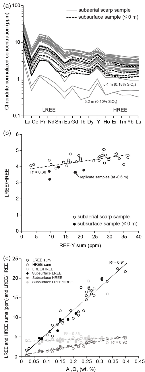
Figure 11. REE-Y elements on the Sparta Fault (Anogia B profile). (a) Concentrations of rare-earth elements and yttrium (REE-Y) normalized to chondrite composition (McDonough and Sun, 1995). Each line shows a measured location on the scarp surface. The two low REE-Y outliers at 5.2 and 5.4 m also have exceptionally low SiO 2 and Al 2 O 3 . (b) LREE : HREE versus REE-Y sum. The R^2 value is for a linear fit. (c) LREE, HREE, and LREE : HREE versus Al 2 O 3 (wt %). The R^2 values are for linear fits. In each panel, the six subsurface samples ( \leq 0 m), including a replicate measurement at -0.6 m, are shown as filled circles.
