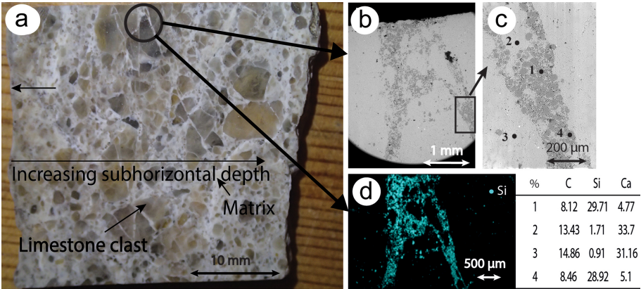
Figure 9. Concentrations of Si in the Sparta Fault breccia, 1.1 m above the scarp base at Anogia. (a) A cut drill core from the Sparta Fault scarp at Anogia showing limestone clasts cemented in fine matrix. The circled fine matrix is examined under high resolution in panels (b) to (d). (b) An ESEM image showing the sample location for spot elemental analysis (rectangle). (c) Sample points for elemental analysis using EDS, with values shown in the table. (d) The abundance of Si in the fine matrix illustrated in magenta for the circled part of the thin section shown in panel (a).
