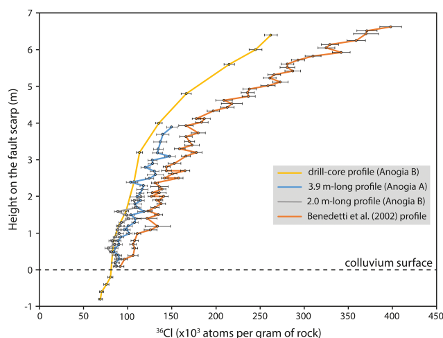
Figure 2. Sparta Fault ^{36}\text{Cl} concentration profiles. Error bars indicate 1\sigma measurement uncertainties.
