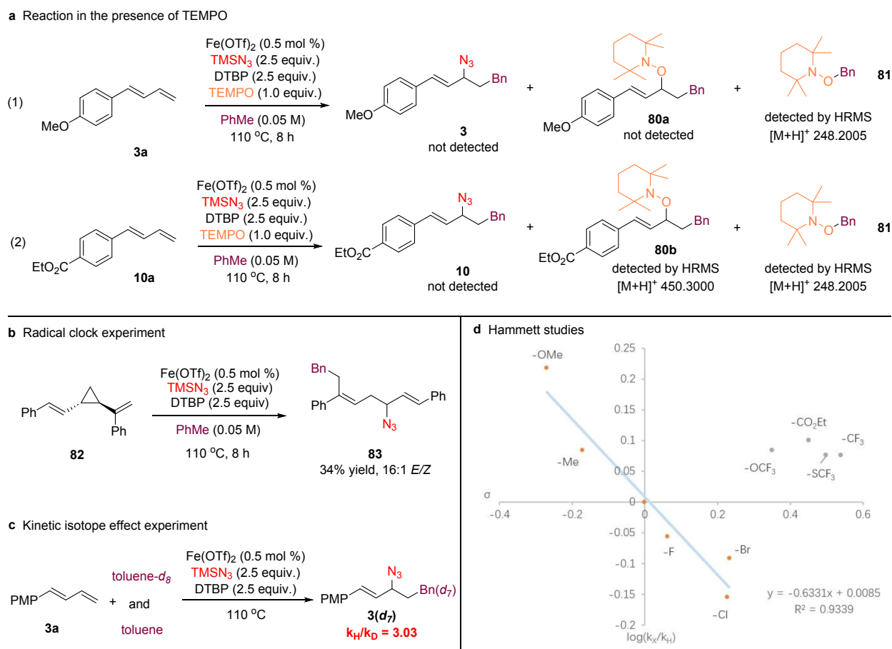
Scheme 3. Mechanistic studies.
