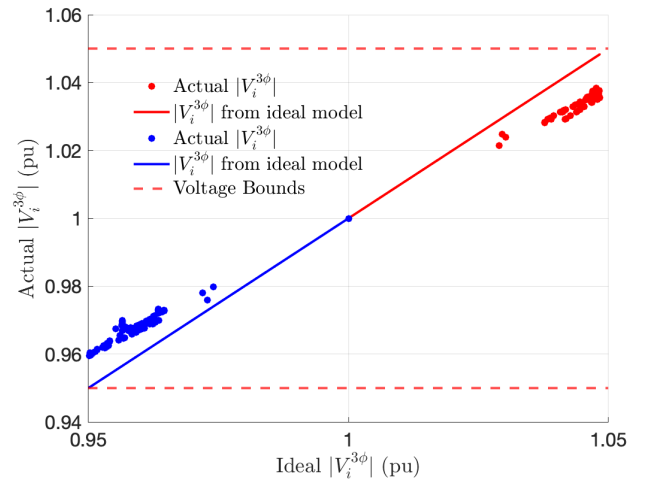
Fig. 2. Comparison of 3-phase voltages in the modified IEEE 37-node system, taking into account mutual impedances (actual) versus ignoring mutual impedances (ideal). In this figure, blue, and red correspond to voltages obtained using \mathbf{P}_{\text{CIA}}^+ , and \mathbf{P}_{\text{CIA}}^- , respectively.
