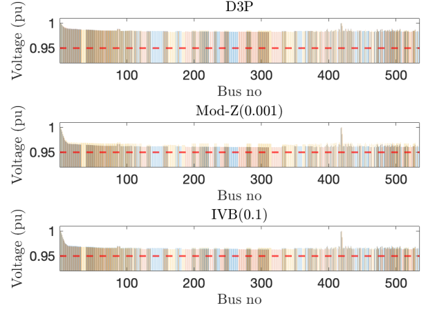
Fig. 8. Voltage profiles for a 534-node feeder are depicted in the figures below for \mathbf{P}_{CIA}^{\phi,-} . In these figures, blue, red, and yellow correspond to phases a, b, and c, respectively.
