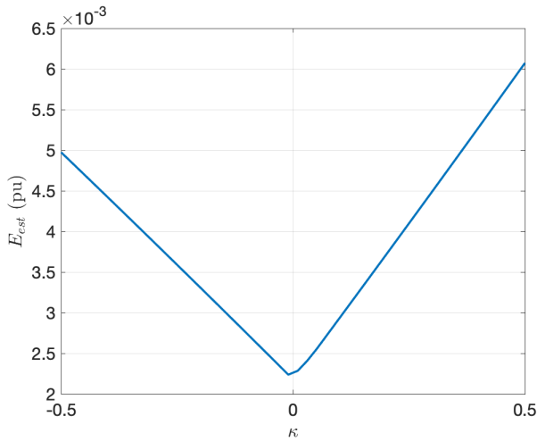
Fig. 4. Illustrating the impact of mutual impedance mismatch on the performance of Mod-Z .
