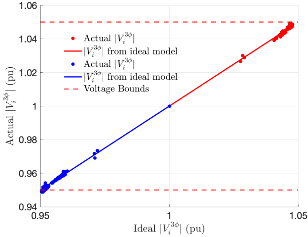
Fig. 3. Voltages magnitudes for the IEEE 37-node system after modifying the impedance matrix based on Mod-Z approach. In this figure, blue, and red correspond to voltages obtained using \mathbf{P}_{CIA}^+ , and \mathbf{P}_{CIA}^- , respectively.
