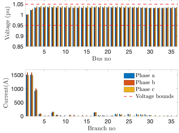
Fig. 1. Illustrating the effects of D3P on 3-phase voltage and current profiles following the addition of nodal injections p_a^+ + p_b^+ + p_c^+ . The dashed red line indicates the ANSI voltage limits of [0.95, 1.05] pu.
