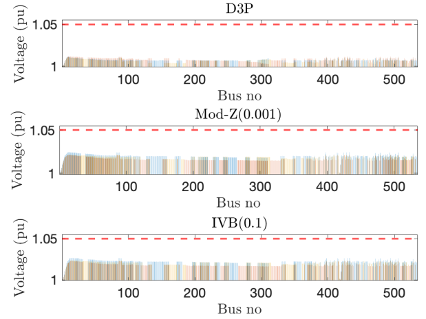
Fig. 9. Voltage profiles for a 534-node feeder are depicted in the figures below for \mathbf{P}_{CIA}^{\phi,+} . In these figures, blue, red, and yellow correspond to phases a, b, and c, respectively.
