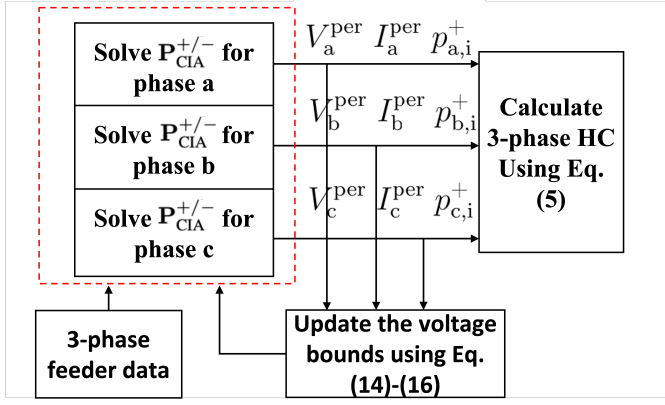
Fig. 5. Flowchart of the proposed IVB approach.
