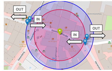
Fig. 3. This sample Counting Experiment map shows four data collectors positioned at a set radius away from the sensor. The sensor is the green central map marker in this example. The red circle is a distance of 30 meters; the blue circle is a distance of 40 meters from the sensor.
