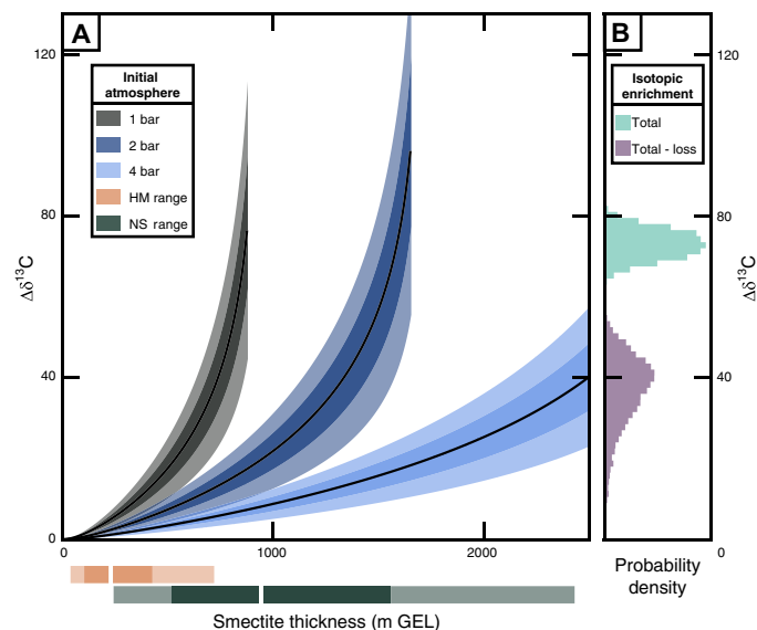
Fig. 2. Predicted change in atmospheric \delta^{13}\text{C} for a variable volume of smectite clays saturated with abiotic methane. (A) Colored segments reflect different initial Martian atmospheric pressures. Data are shown with median (black line), 1 SD (near-opaque field), and 2 SDs (semitransparent field). The orange and green boxes reflect the one and two standard deviation estimates of smectite clay thickness as shown in Fig. 1. (B) Probability density of changes in \delta^{13}\text{C} for the total enrichment since 4.5 Ga (turquoise) and the total enrichment that cannot be explained by current estimates of atmospheric loss alone (purple).
