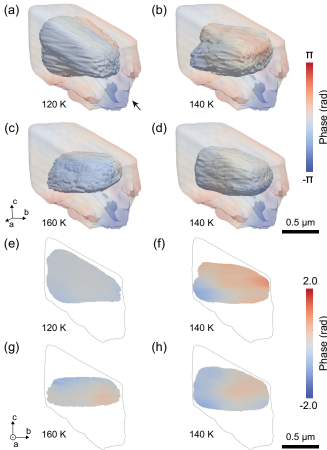
FIG. 4. (a)–(c) Antiferromagnetic domain obtained at T = 120 , 140 , and 160 K, respectively. (d) Antiferromagnetic domain at T = 140 K after the thermal cycling. Translucent images of the crystal from the (116) peak and isosurface images from the antiferromagnetic (106) peak are superimposed. (e)–(h) Corresponding center slice of (a)–(c). Here, the black lines show the profile of the \text{Sr}_2\text{IrO}_4 crystal. The antiferromagnetic images were contoured at 25% of the maximum amplitude and colored according to the image phase at the surface.
